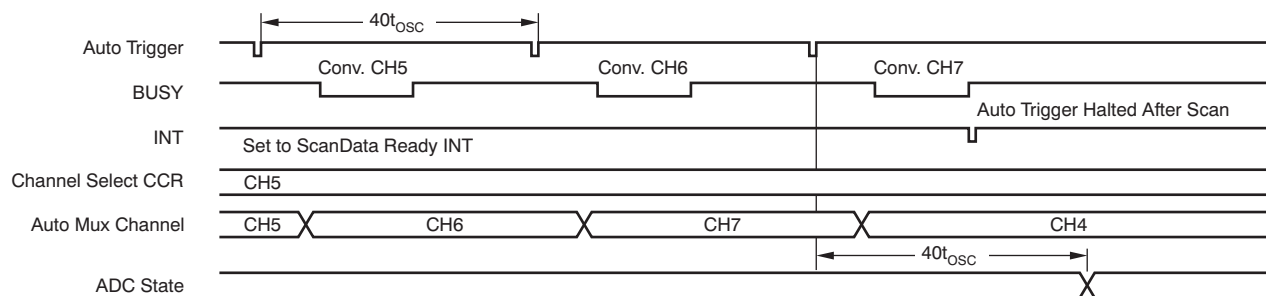
Figure 23. Mode 5 Timing
