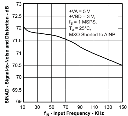
Figure 30. Signal-to-Noise + Distortion vs Input Frequency
