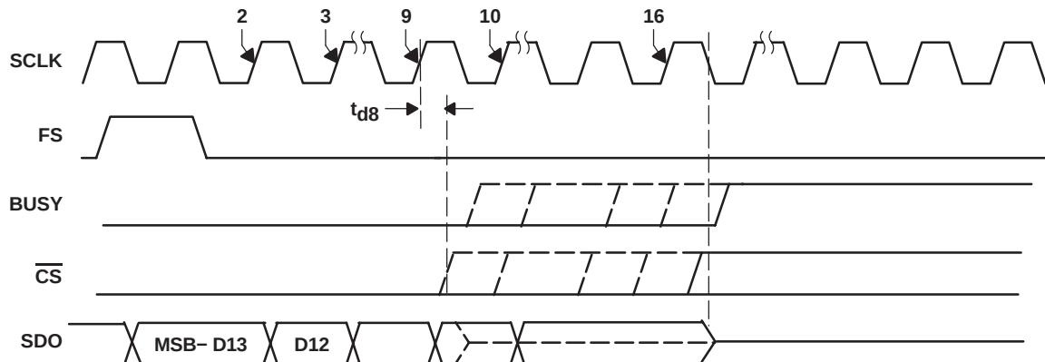
Figure 11. Frame Abort Using \overline{CS} During Sample
