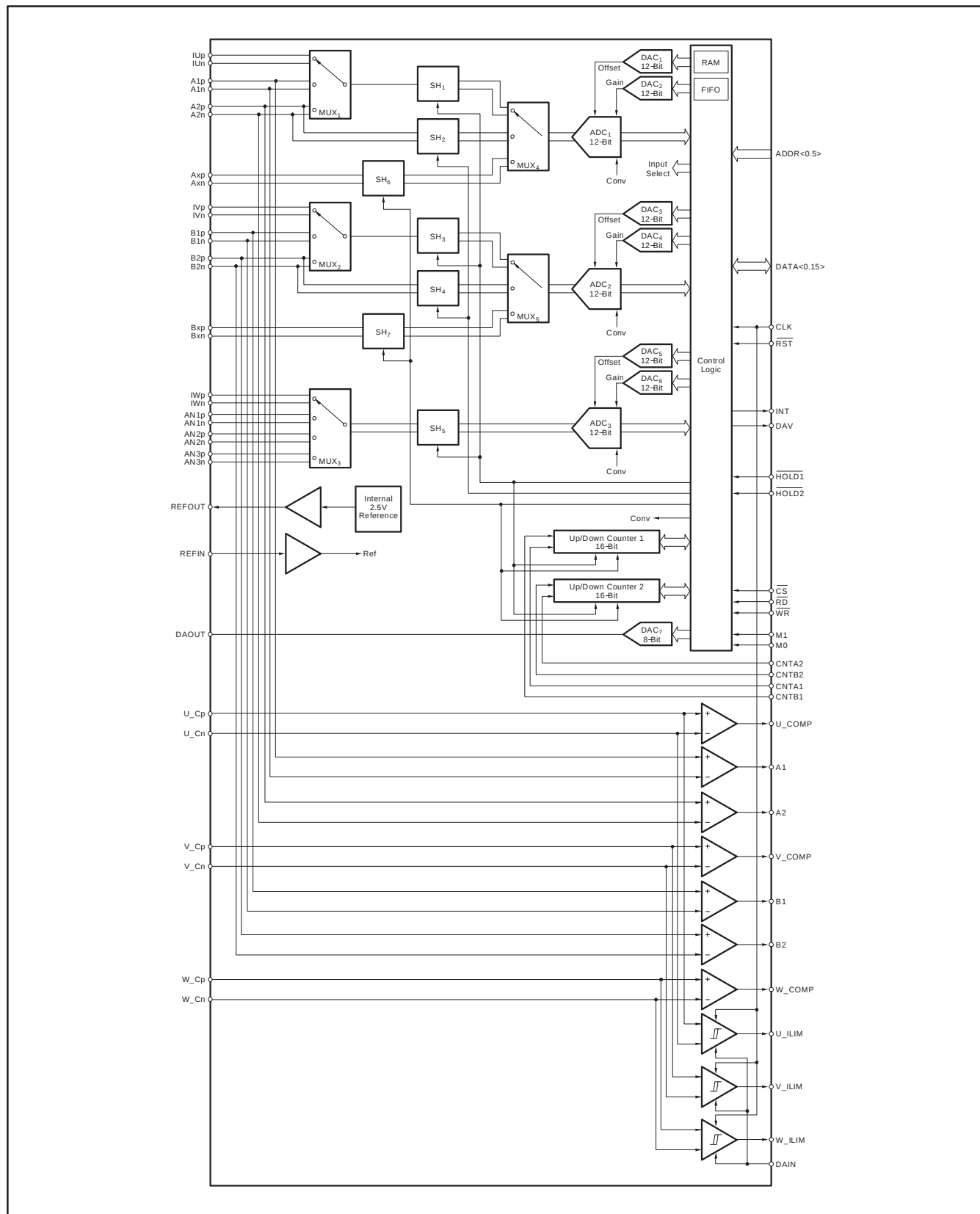
Figure 1–2. Functional Diagram
