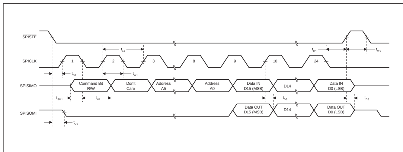
Figure 1–13. SPI Access
