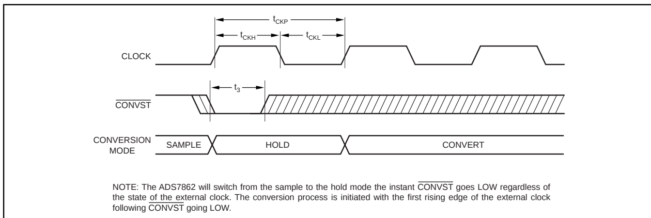
FIGURE 8. Conversion Mode.
