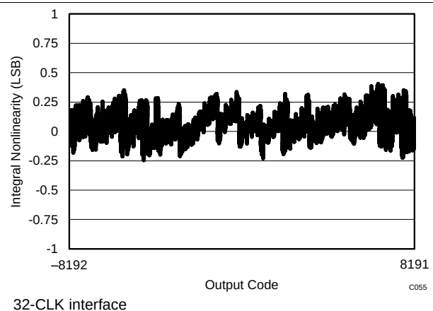
Figure 47. Typical INL
