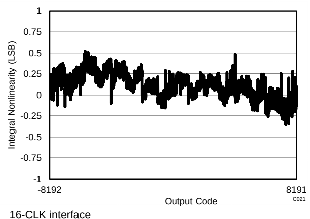
Figure 45. Typical INL
