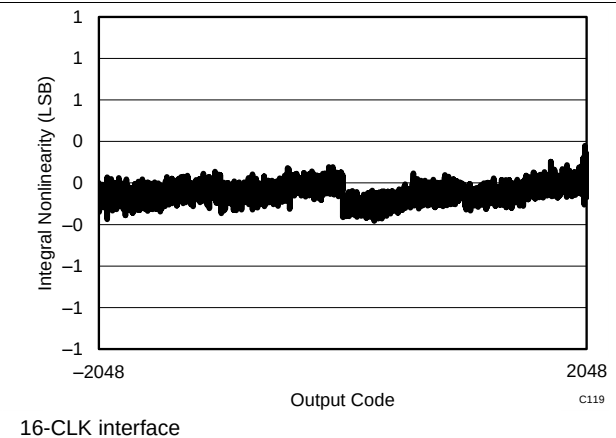
Figure 73. Typical INL
