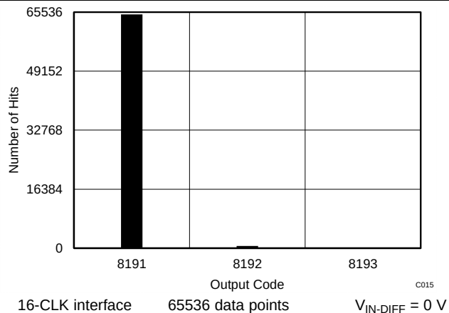
Figure 40. DC Histogram
