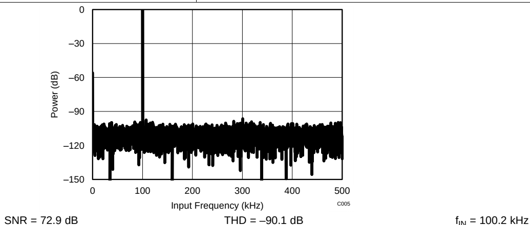
Figure 112. ADS7254 in 32-CLK Interface Mode
