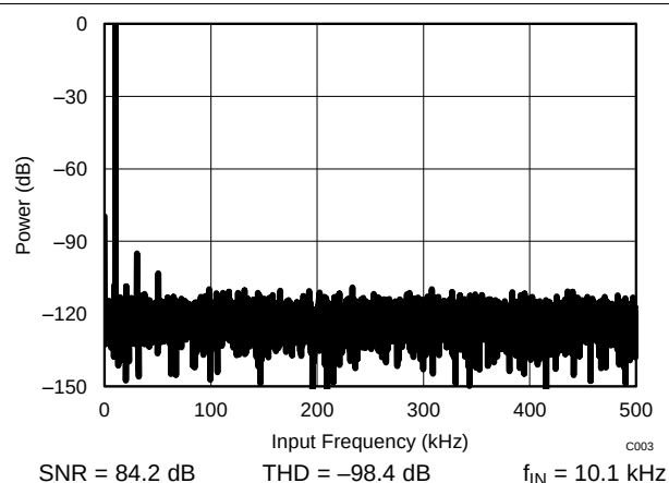
Figure 104. ADS7854 in 32-CLK Interface Mode
