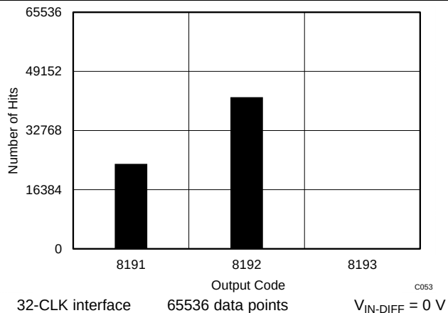
Figure 41. DC Histogram
