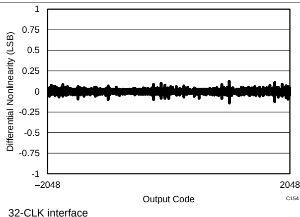
Figure 74. Typical DNL
