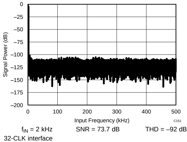
Figure 54. Typical FFT
