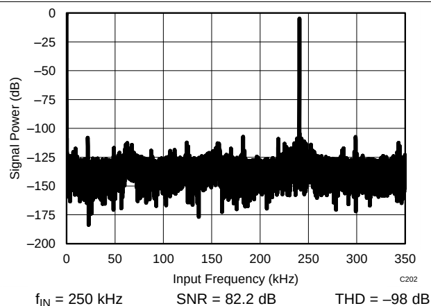
Figure 3. Typical FFT
