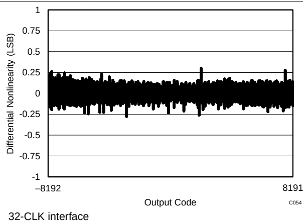
Figure 46. Typical DNL
