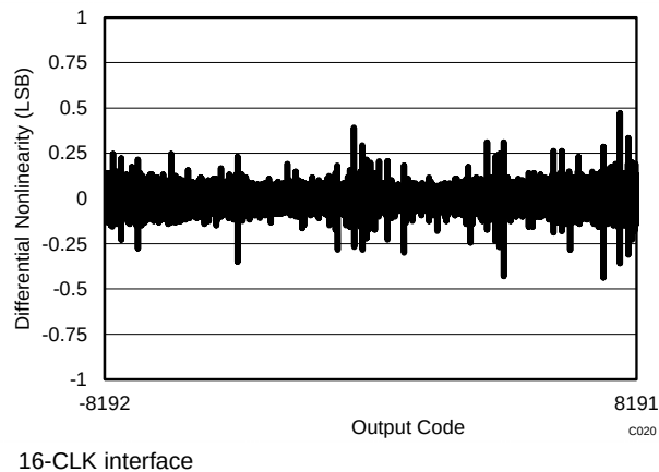
Figure 44. Typical DNL
