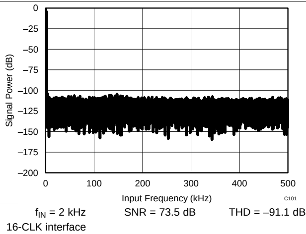
Figure 52. Typical FFT
