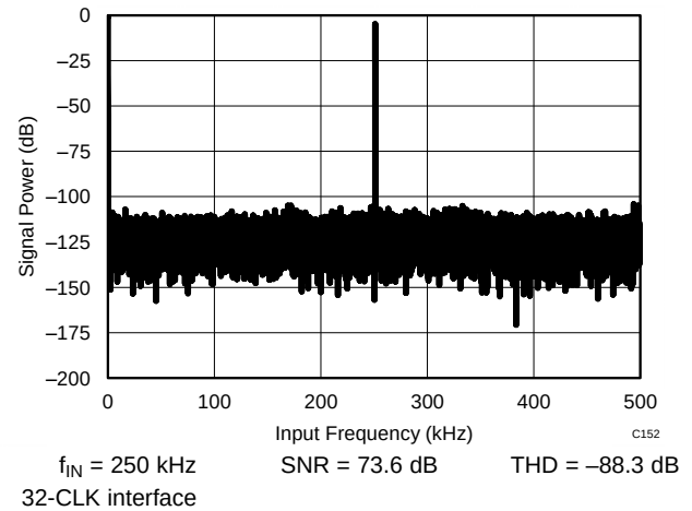
Figure 55. Typical FFT
