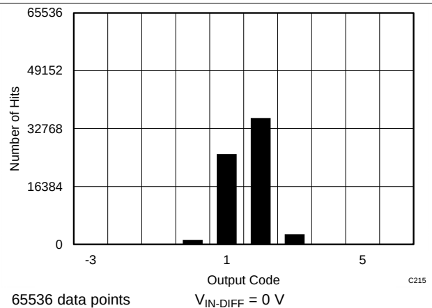
Figure 13. DC Histogram
