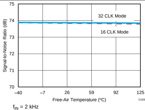
Figure 56. SNR vs Temperature
