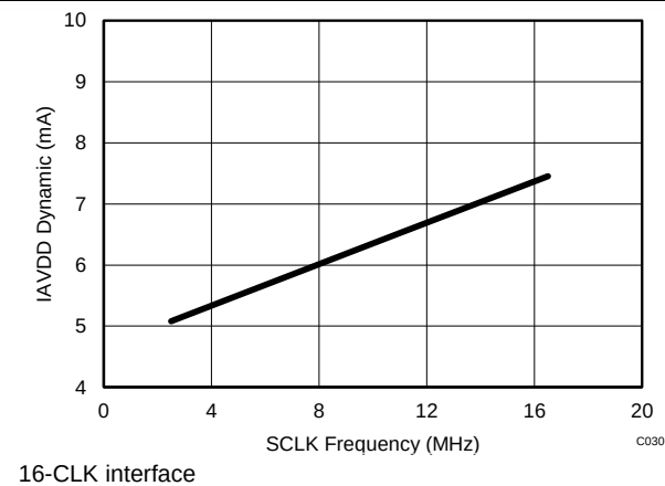
Figure 66. Analog Supply Current vs SCLK Frequency
