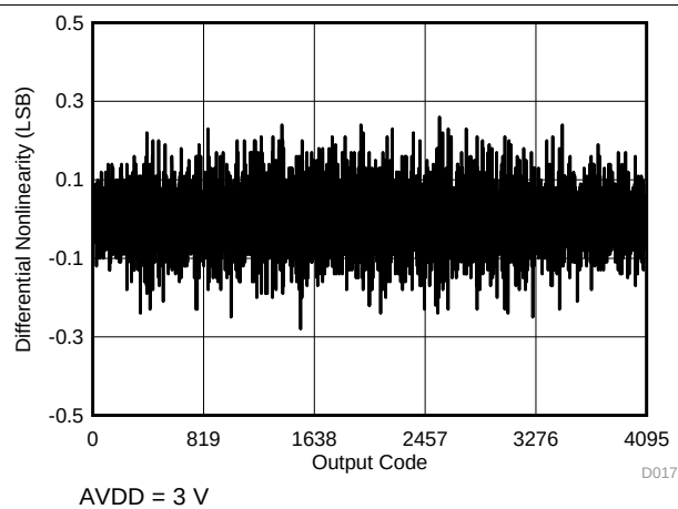
FIG 17. Typical DNL in Manual Mode
