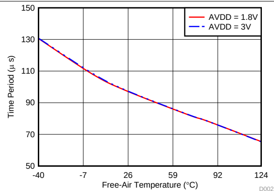
Figure 4. Low Power Oscillator Time Period with Temperature
