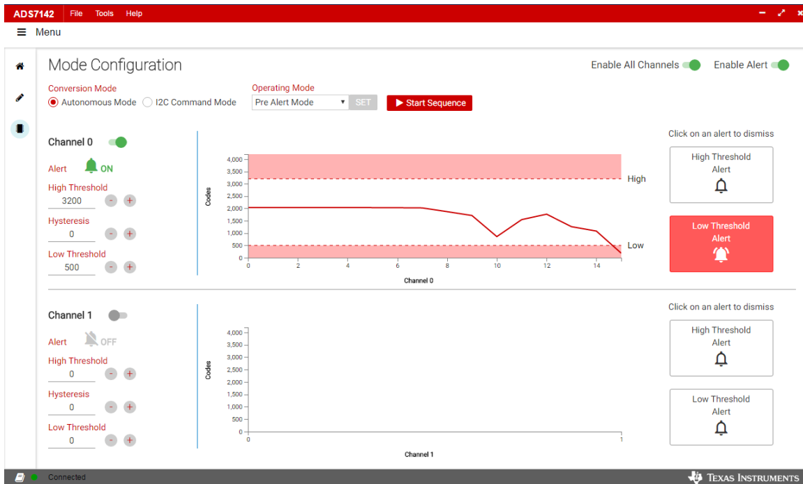
✎ 117. Pre-Alert Data Capture
