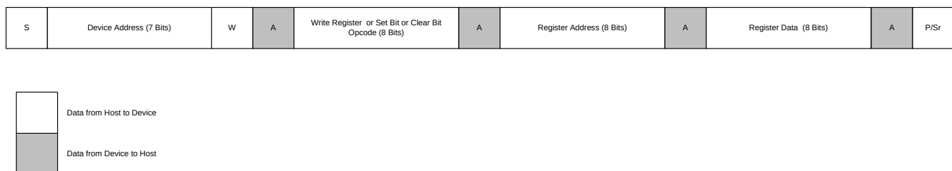
FIG 52. Writing a Single Register
