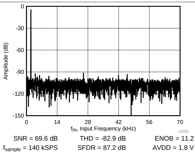
Figure 5. Typical FFT in Manual Mode
