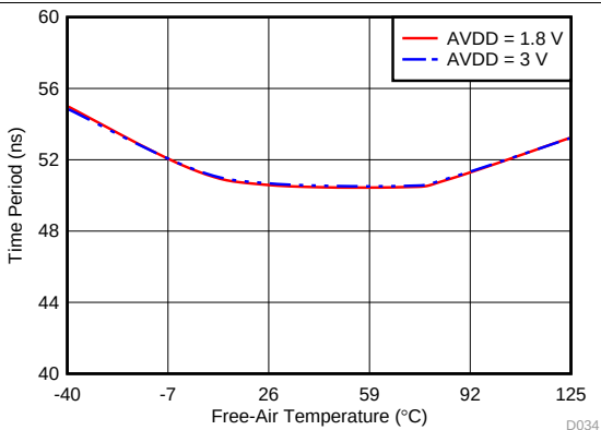
Figure 3. High Speed Oscillator Time Period with Temperature
