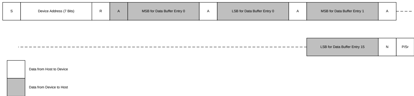
Figure 46. Reading Data Buffer (16 Bit Words × 16 Words)
