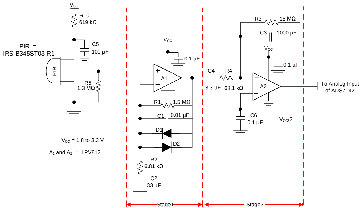
✎ 120. Signal Conditioning Circuit for PIR Sensor
