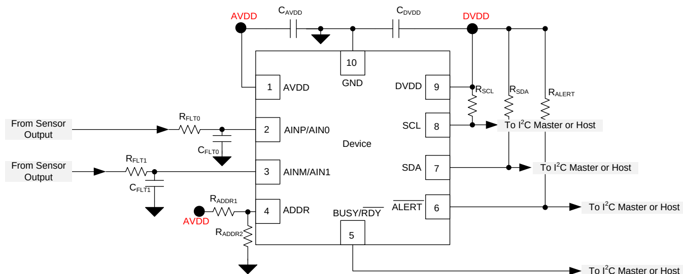
Figure 123. Example Circuit
