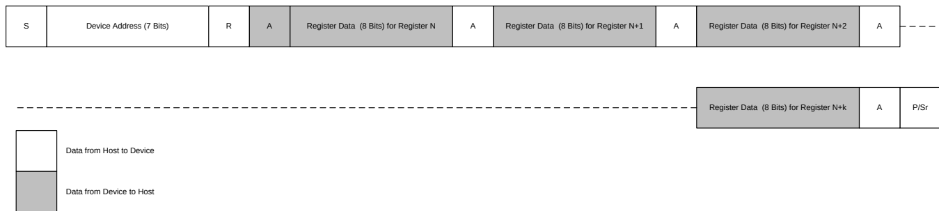
FIG 51. Reading a Continuous Block of Registers
