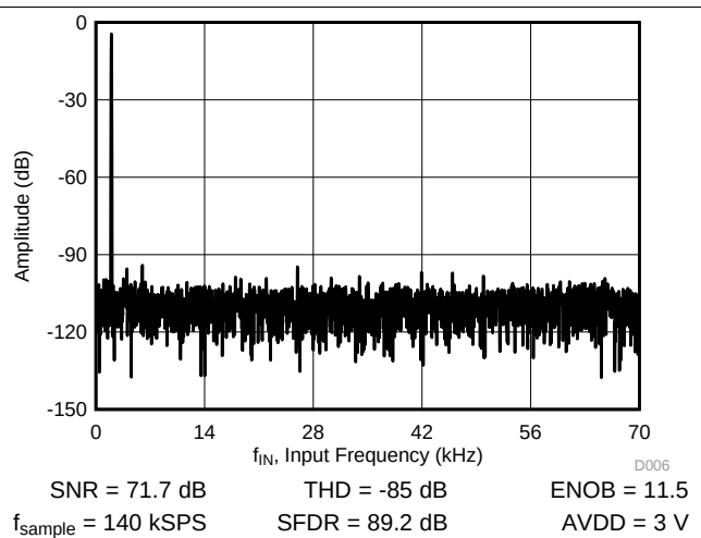
Figure 6. Typical FFT in Manual Mode
