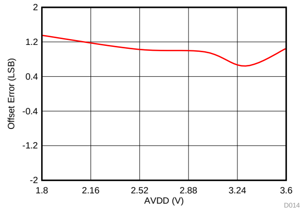
FIG 14. Offset Error in Manual Mode with AVDD
