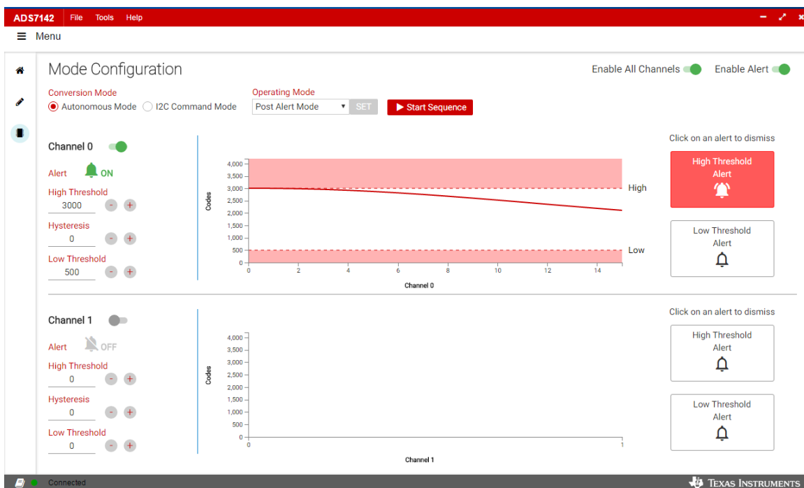
✎ 118. Post Alert Data Capture
