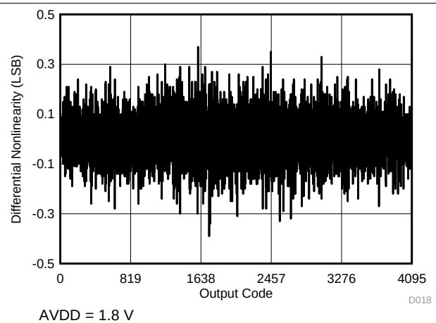
FIG 18. Typical DNL in Manual Mode
