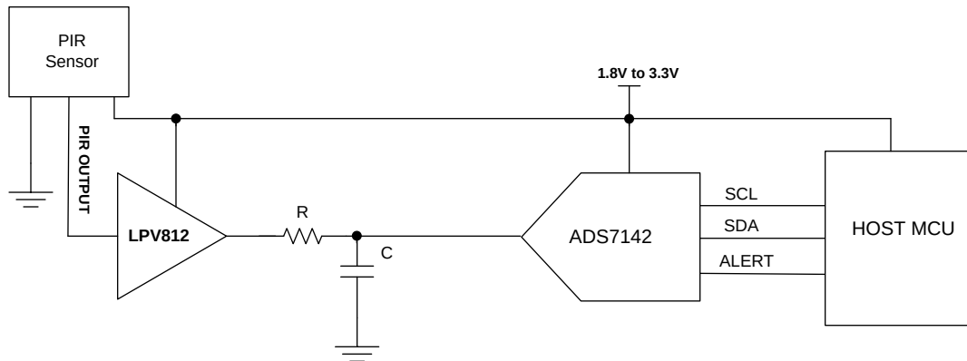
✎ 119. PIR Sensor with ADS7142
