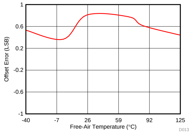
FIG 13. Offset Error in Manual Mode with Temperature
