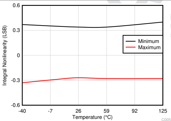
FIG 7-4. Typical INL
