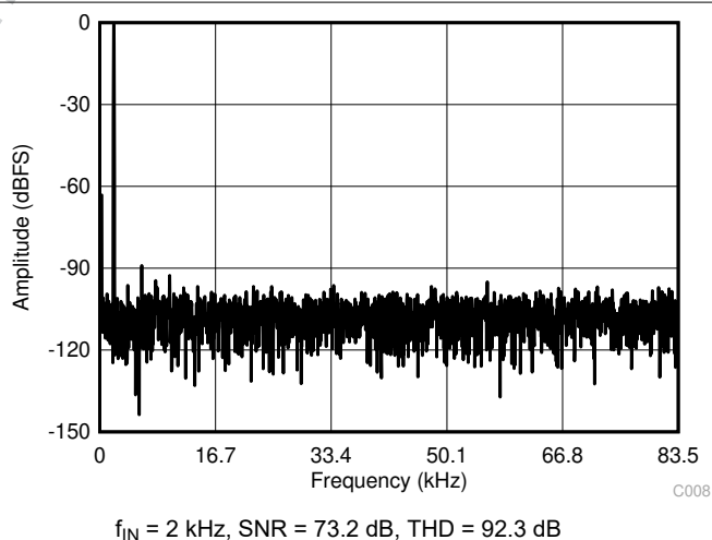
FIG 7-13. Typical FFT
