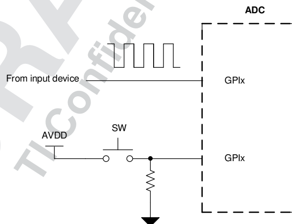
FIG 9-2. Digital Input
