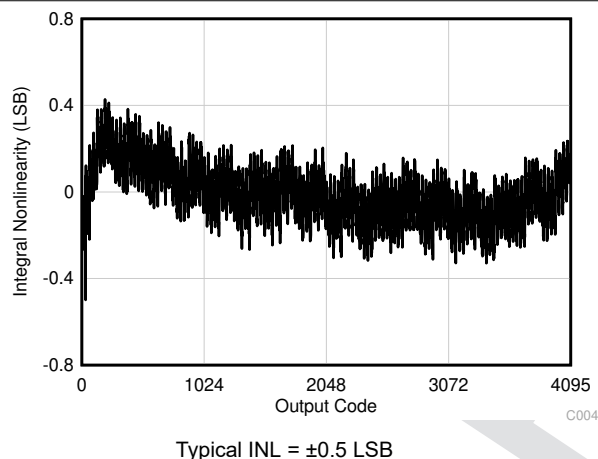
FIG 7-4. Typical INL
