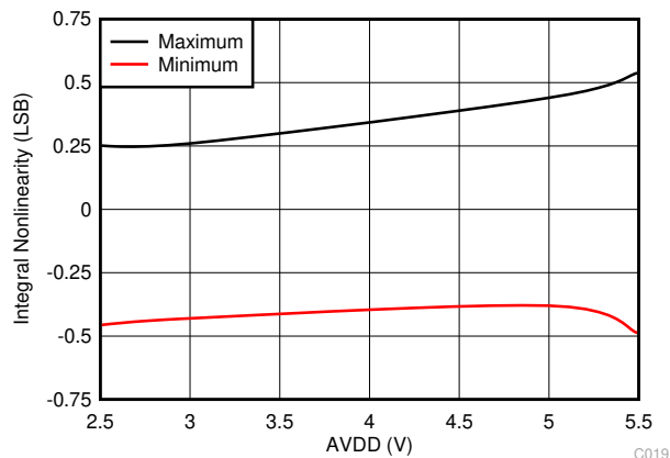
FIG 7-8. INL vs AVDD
