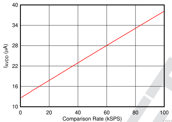
FIG 7-22. Analog Supply Current vs Comparison Rate (OSC_SEL = 1) in Turbo Comparator Mode
