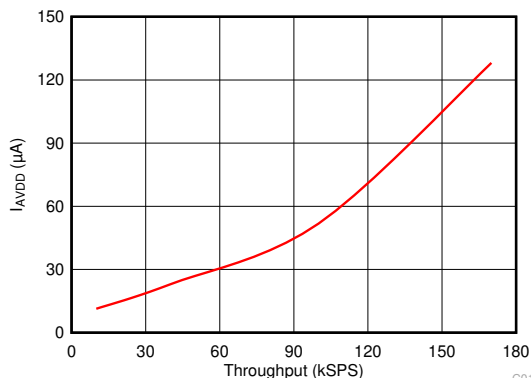
FIG 7-20. Analog Supply Current vs Throughput
