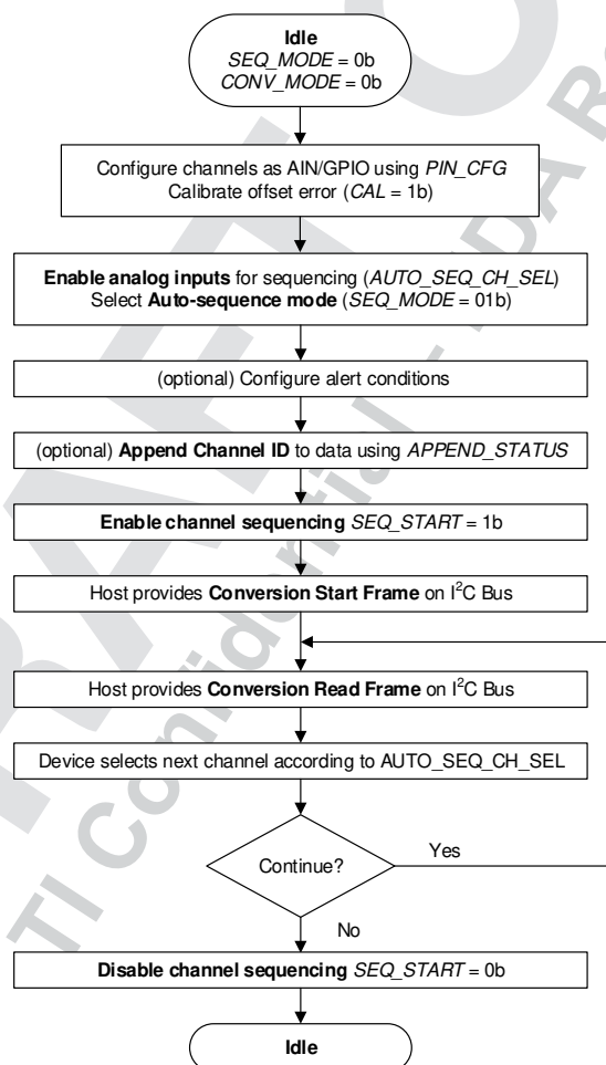
FIG 8-14. Device Operation in Auto-Sequence Mode
