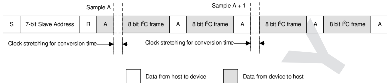
FIG 8-13. Starting a Conversion and Reading Data in Manual Mode
