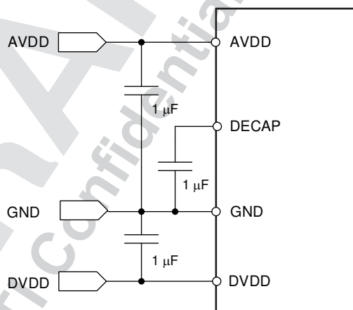
Figure 10-1. Power-Supply Decoupling
