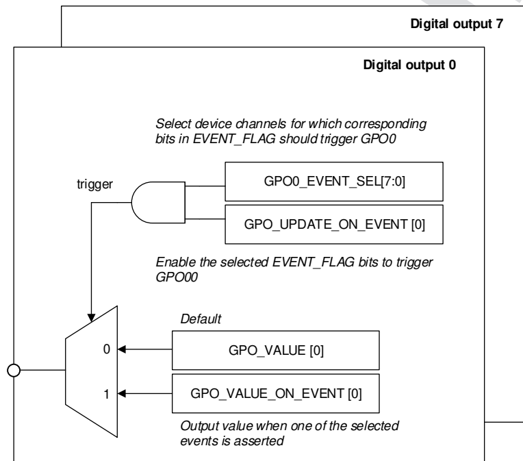
図 8-11. Block Diagram of the Digital Output Logic
