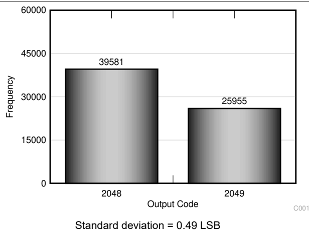
FIG 7-2. DC Input Histogram
