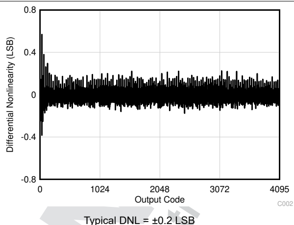
FIG 7-3. Typical DNL
