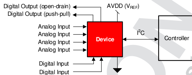
FIG 9-1. DAQ Circuit: Single-Supply DAQ
