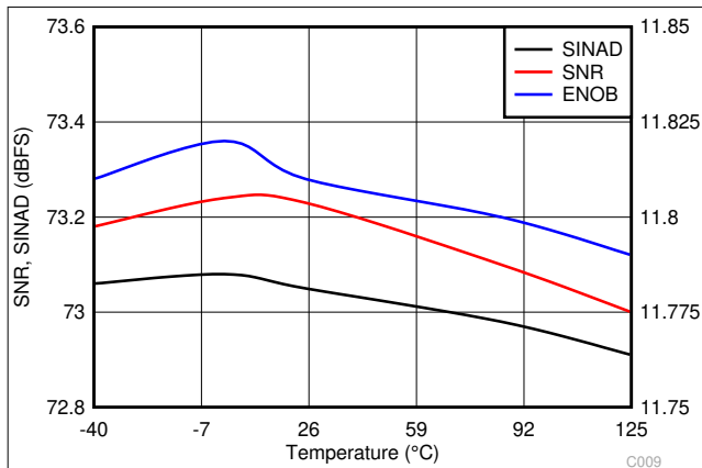
Figure 7-14. Noise Performance vs Temperature
