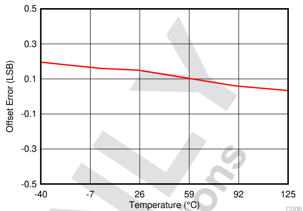
FIG 7-9. Offset Error vs Temperature
