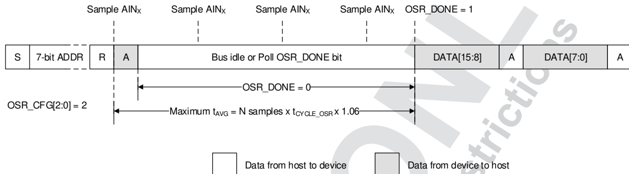
Figure 8-4. Averaging Example
