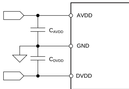
Figure 52. Power-Supply Decoupling
