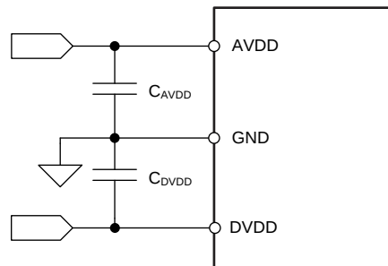
Figure 47. Power-Supply Decoupling
