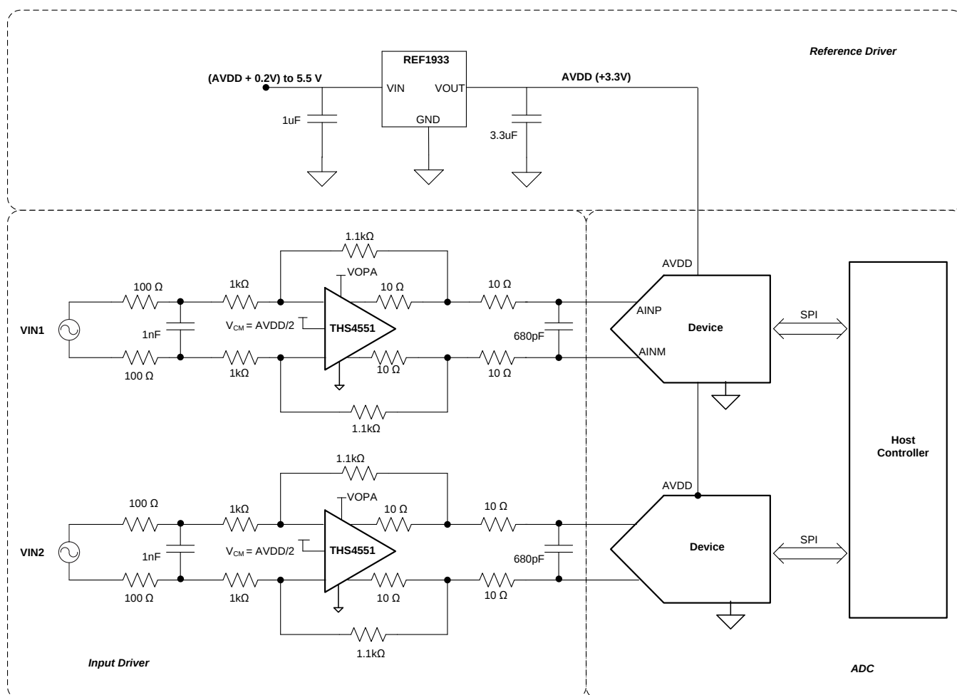
Figure 40. 2-Channel, Simultaneous-Sampling Data Acquisition (DAQ) Circuit Using the ADS7047
