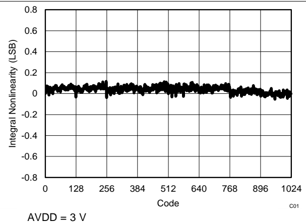
Figure 19. Typical INL
