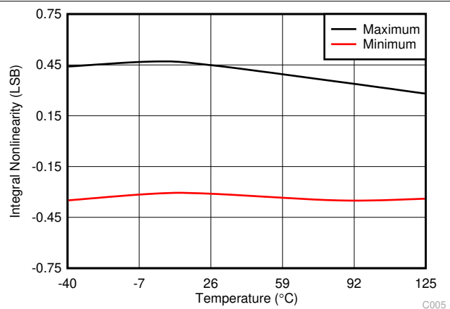
Figure 7-6. Typical INL
