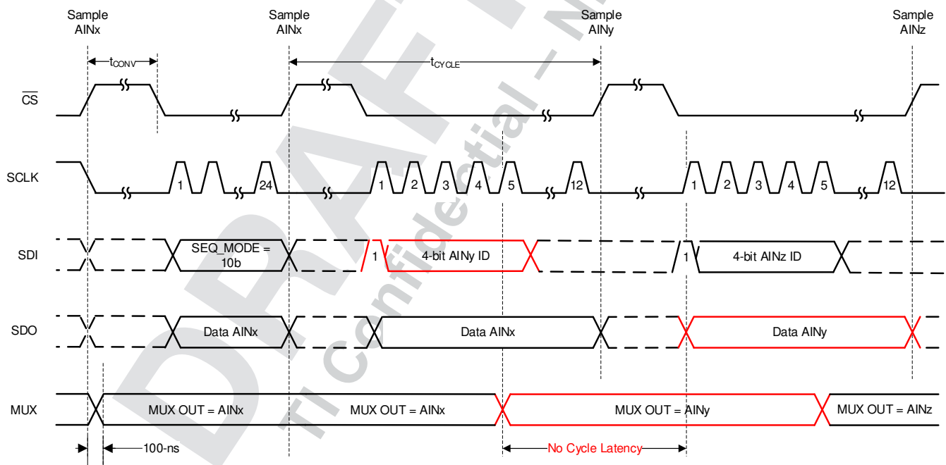
FIG 8-16. Starting Conversions and Reading Data in On-the-Fly Mode
