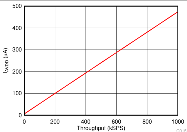
FIG 7-21. Analog Supply Current vs Throughput
