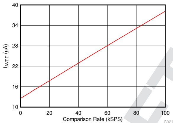
FIG 7-21. Analog Supply Current vs Throughput
