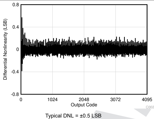
Figure 7-5. Typical DNL
