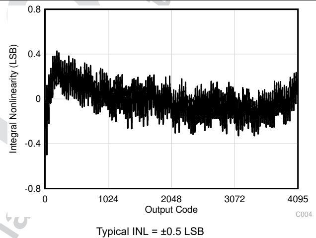
Figure 7-6. Typical INL
