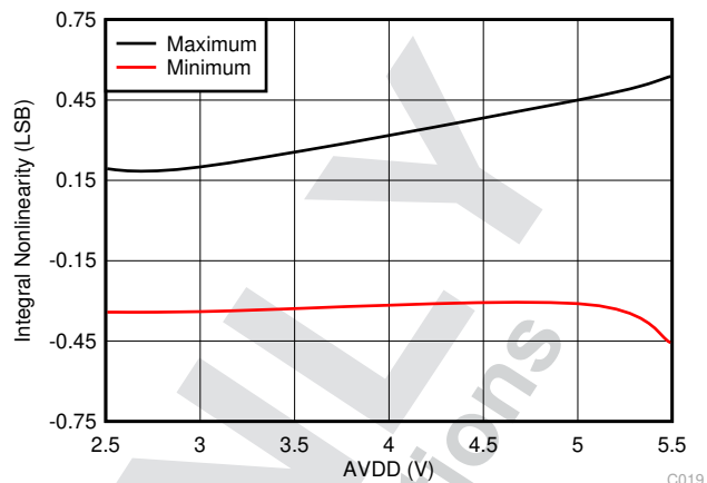
FIG 7-10. INL vs AVDD
