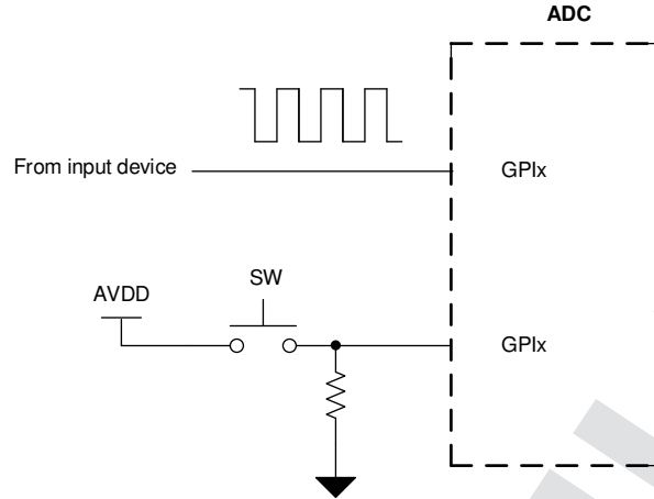
FIG 9-2. Digital Input
