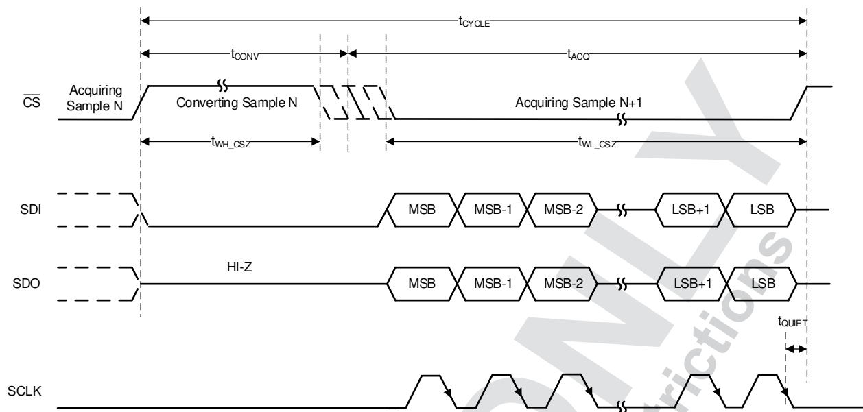
7-1. Conversion Cycle Timing
