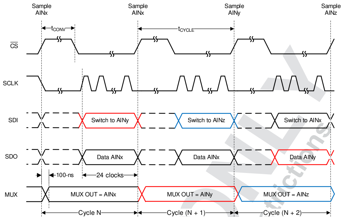
FIG 8-15. Starting Conversions and Reading Data in Manual Mode
