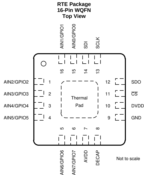
Pin Functions
