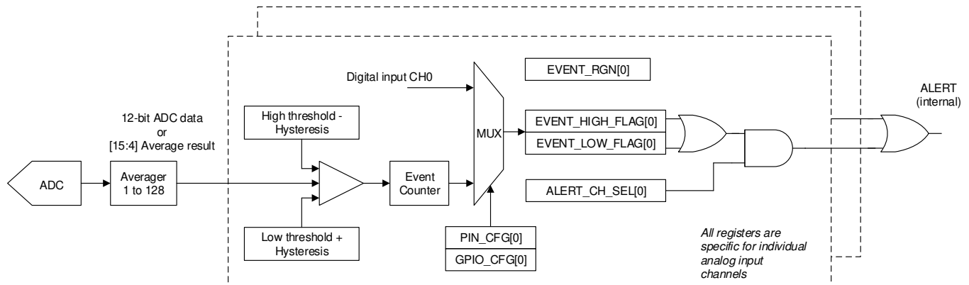
Figure 8. Digital Window Comparator Block Diagram
