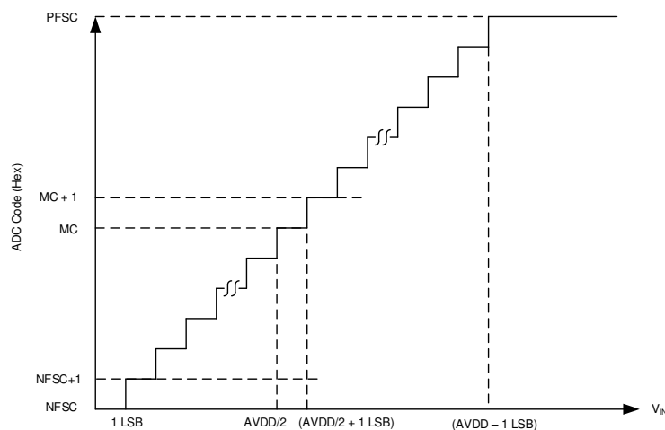
図 4. Ideal Transfer Characteristics
