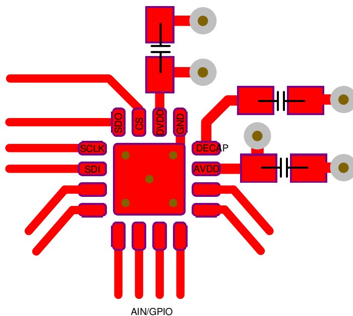
Figure 142. Example Layout
