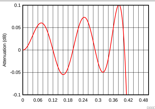
Figure 41. Decimation Filter Response Passband Ripple Detail
