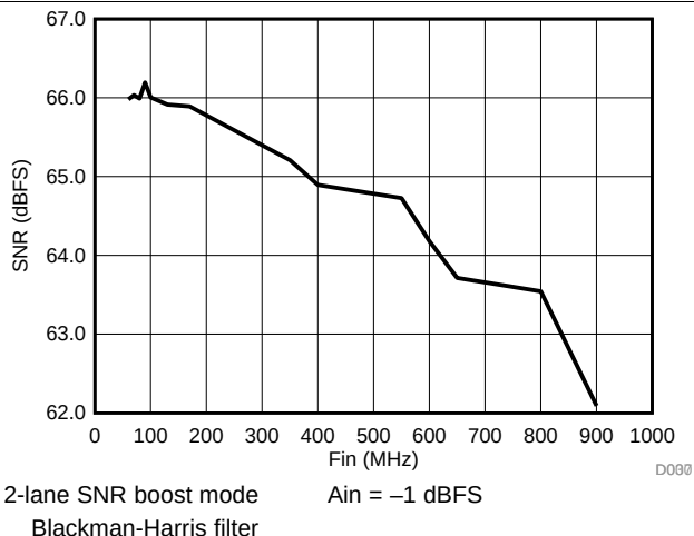
Figure 35. SNR Boost SNR vs. Frequency
