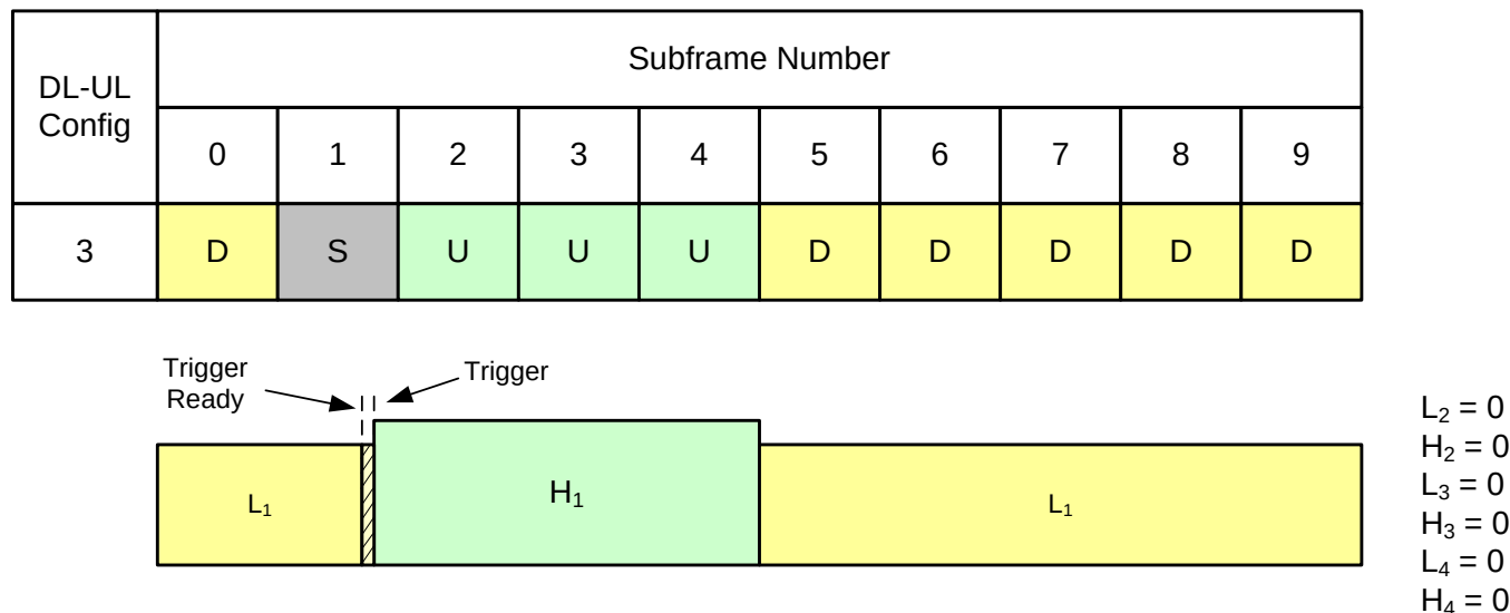
Figure 61. TDD Burst Mode Example 2
