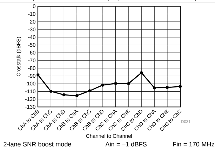
Figure 36. SNR Boost Crosstalk by Channel
