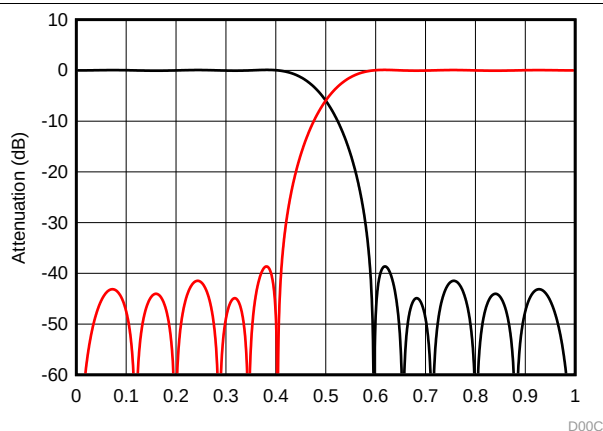
Figure 40. Decimation Filter Response
