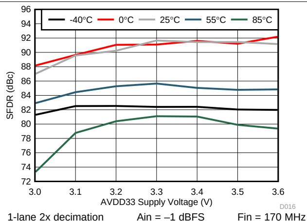
Figure 20. SFDR vs. AVDD33
