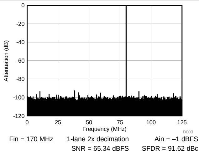
Figure 8. FFT 170 MHz
