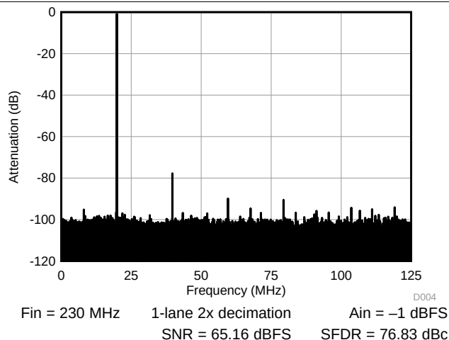
Figure 9. FFT 230 MHz
