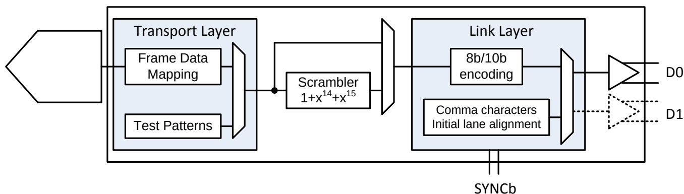
Figure 45. JESD204B Block
