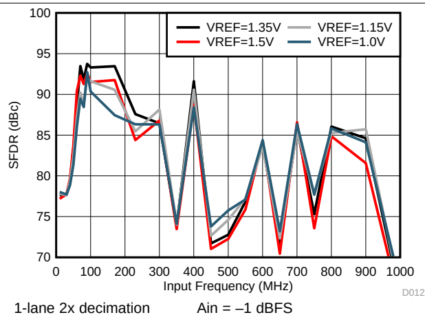
Figure 16. SFDR vs. VREF
