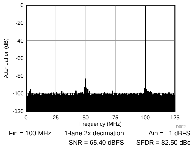
Figure 7. FFT 100 MHz
