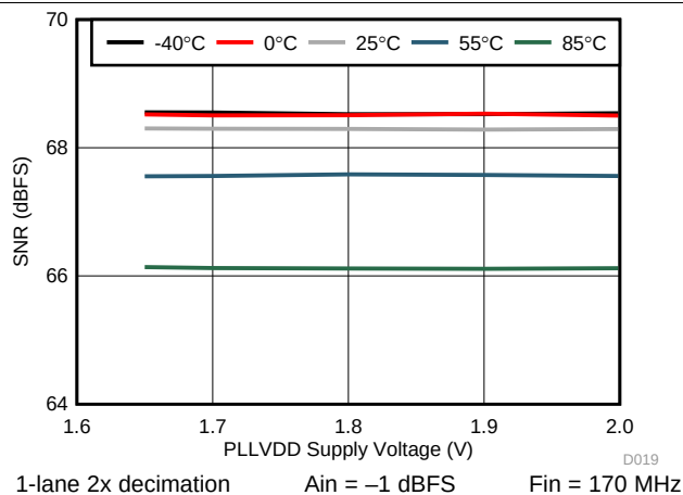
Figure 23. SNR vs. PLLVDD
