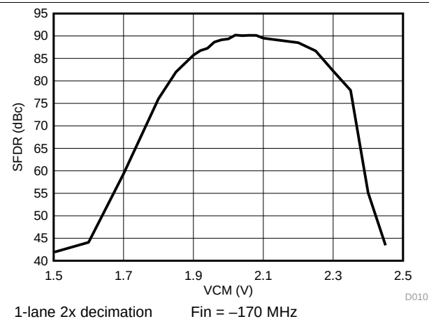
Figure 14. SFDR vs. VCM
