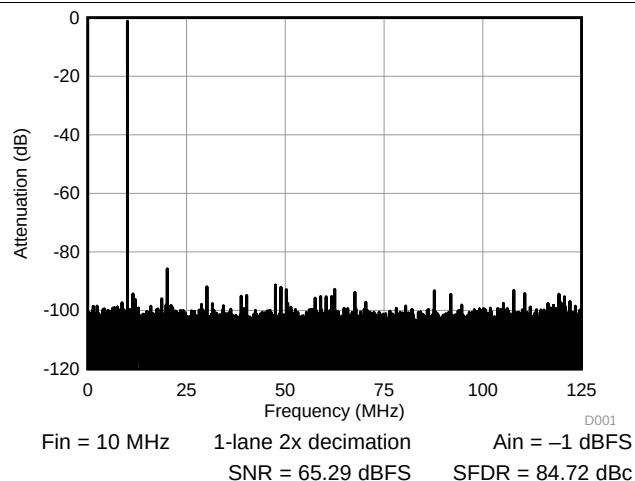
Figure 6. FFT 10 MHz
