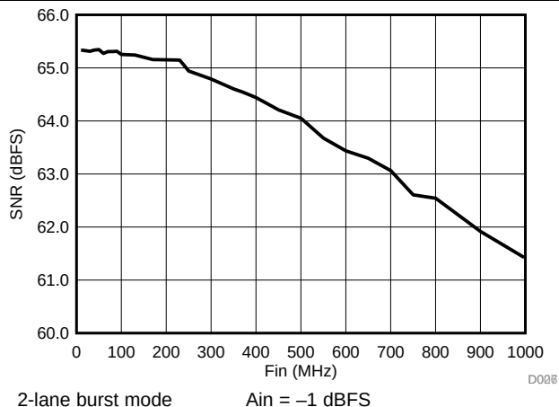
Figure 31. Burst Mode SNR vs. Frequency
