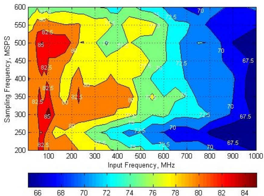
Figure 38. SFDR Contour Plot
