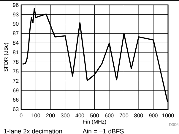
Figure 10. SFDR vs Frequency
