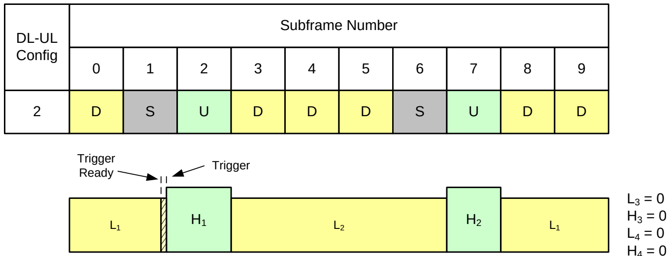
Figure 60. TDD Burst Mode Example 1
