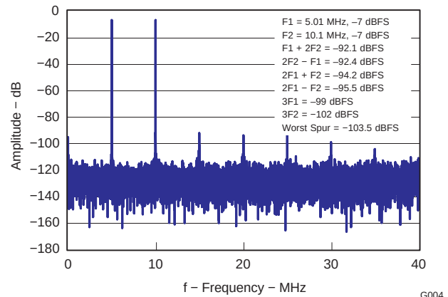
Figure 9. Intermodulation Distortion
