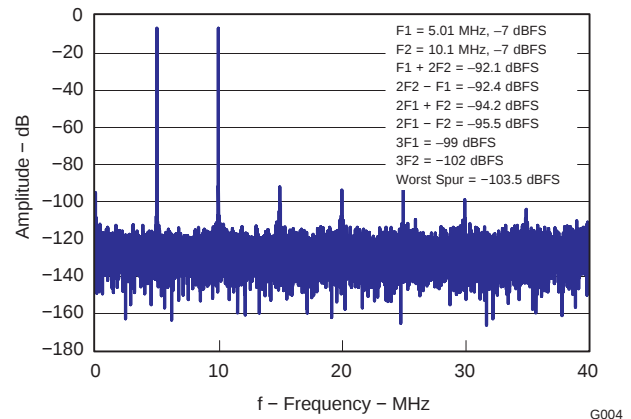
Figure 9. Intermodulation Distortion
