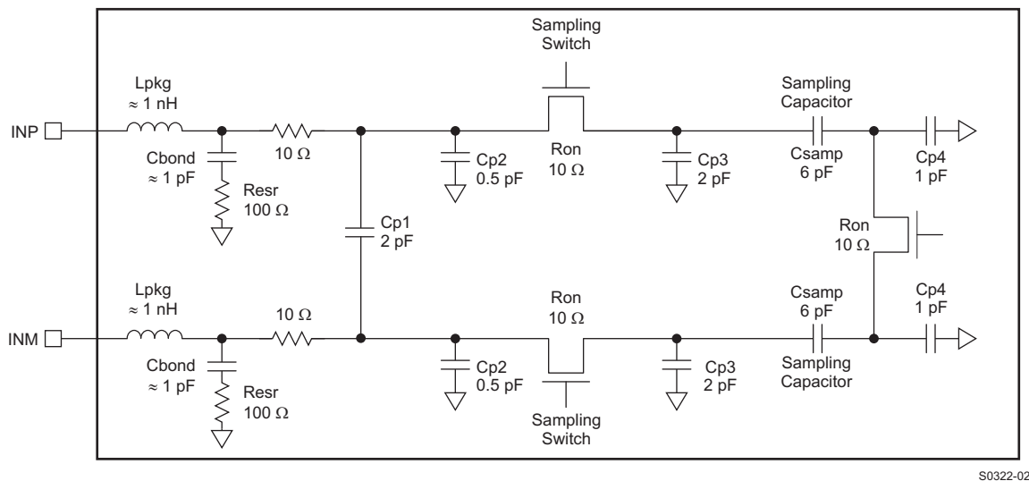
Figure 45. Input Stage
