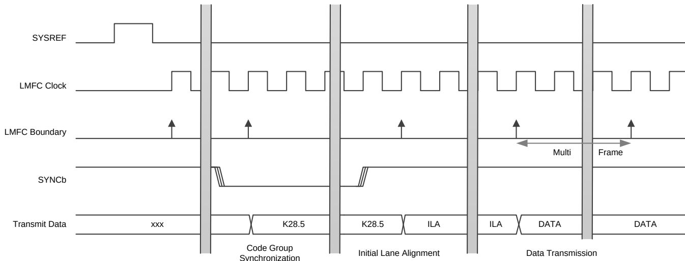
Figure 67. ILA Sequence
