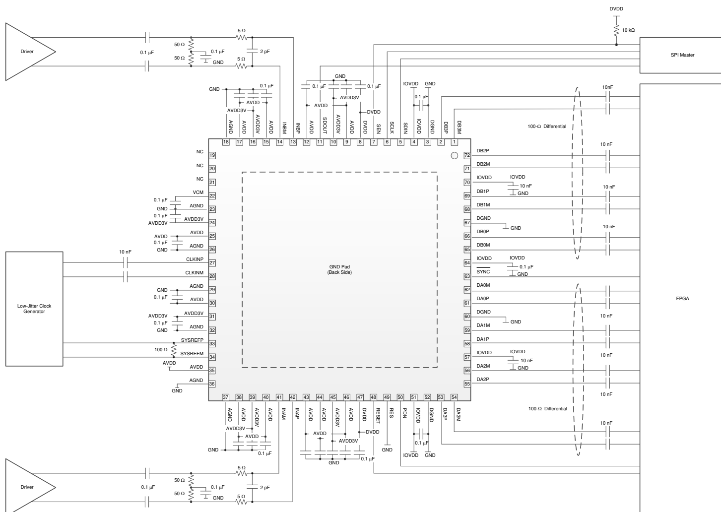
9-14. AC-Coupled Receiver
