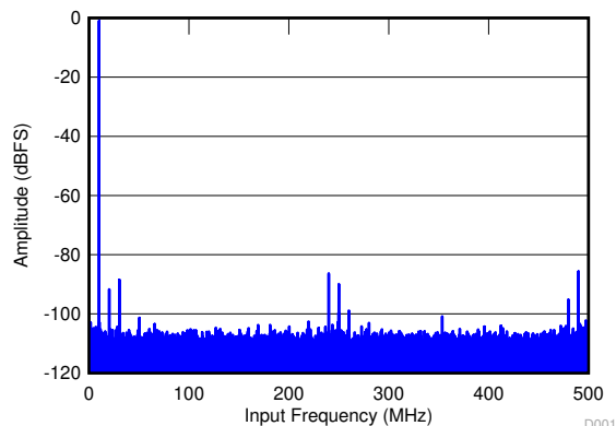
FIG 7-3. FFT for 10-MHz Input Signal
