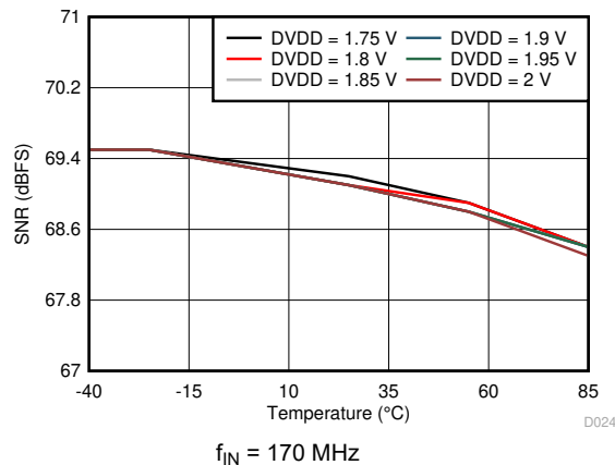
Figure 7-27. Signal-to-Noise Ratio vs DVDD Supply and Temperature
