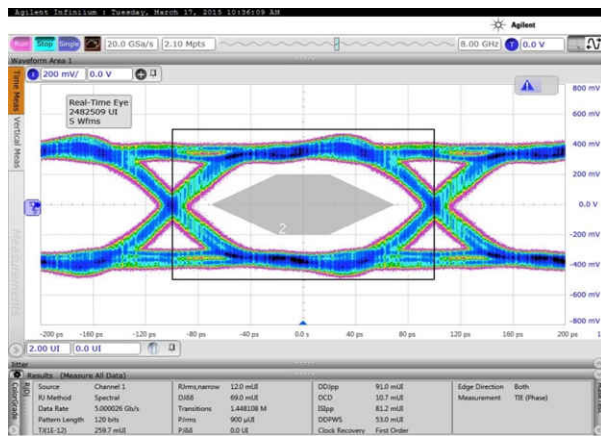
8-23. Eye at 5-Gbps Bit Rate with Default Output Swing
