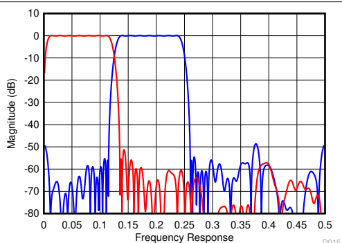
图 8-6. Decimate-by-4 Filter Response
