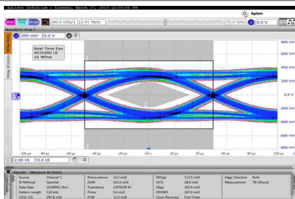
8-25. Eye at 10-Gbps Bit Rate with Default Output Swing
