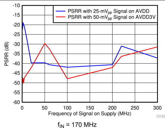
7-44. Power-Supply Rejection Ratio vs Test Signal Frequency
