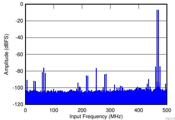
f_{IN1} = 470 \text{ MHz} , f_{IN2} = 465 \text{ MHz} , each tone at -7 \text{ dBFS} , \text{IMD3} = 74.9 \text{ dBFS}
