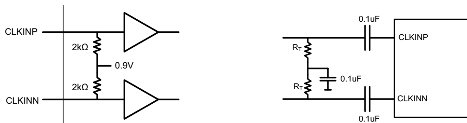
Figure 37. Recommended Differential Clock Driving Circuit
