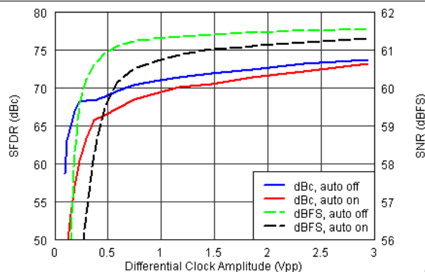
Figure 26. Performance Across Clock Amplitude
