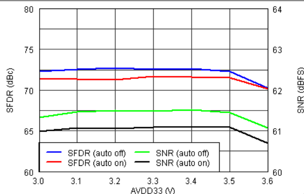
Figure 24. Performance Across AVDD33 ( f_{\text{in}} = 230\text{ MHz} )
