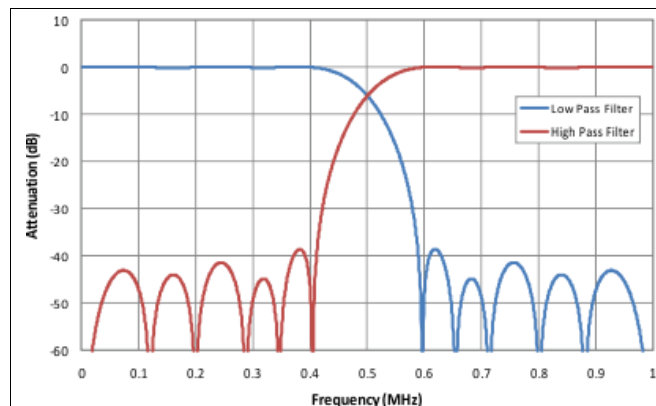
Figure 42. Decimation Filter Response
