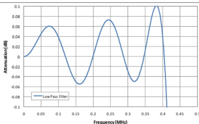
Figure 43. Decimation Filter Response
