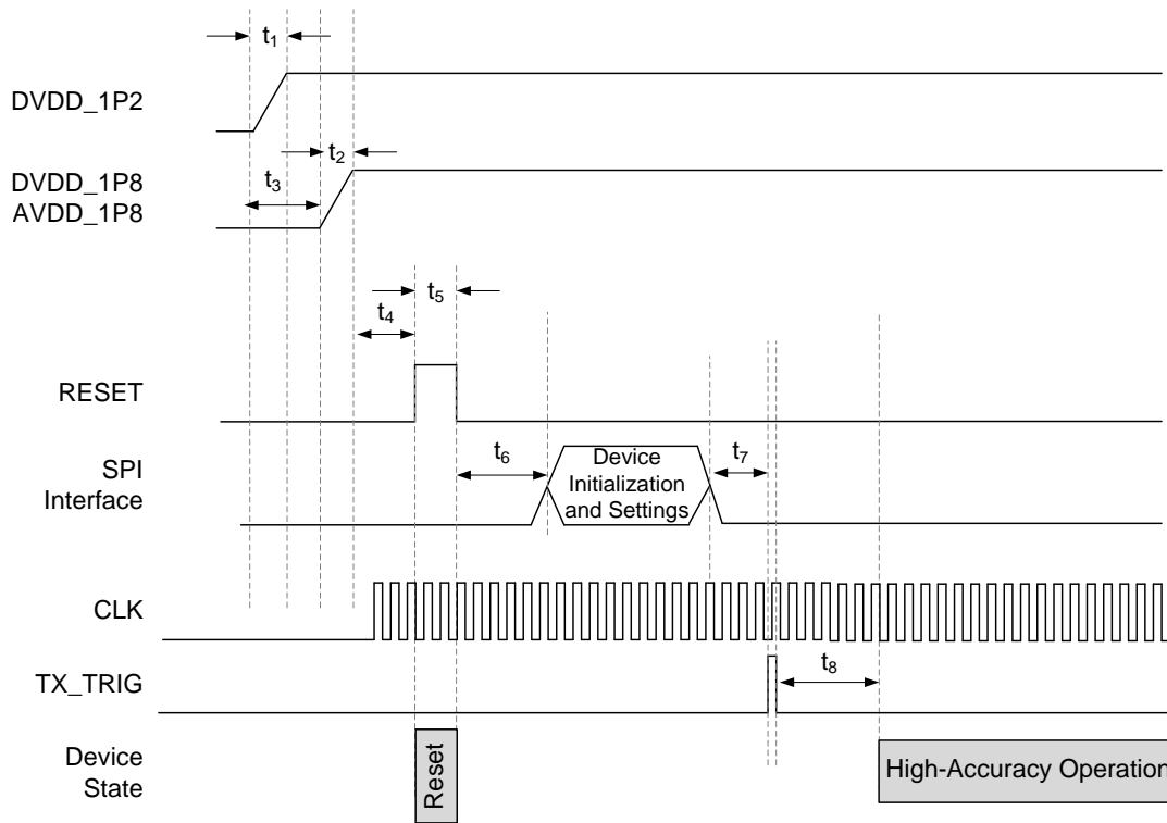
図 95. Power Sequencing and Initialization
