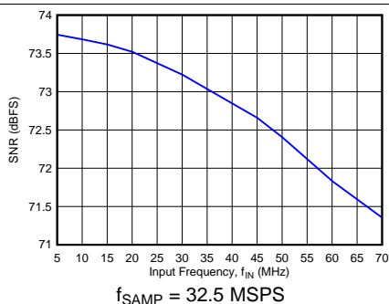
FIG 14. Signal-to-Noise Ratio vs f_{IN} in 14-Bit, 32-Input Mode
