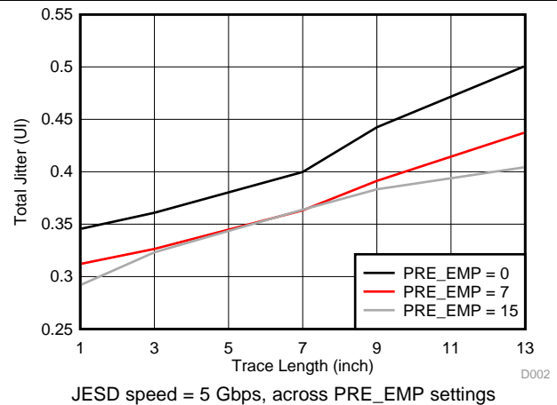
FIG 41. Total Jitter vs Trace Length
