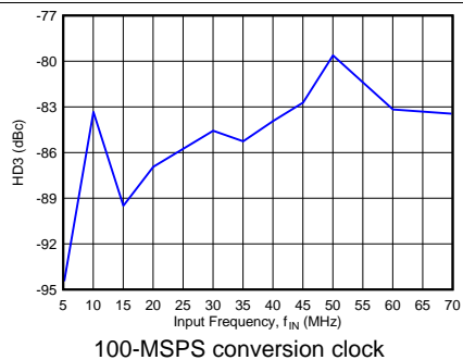
FIG 16. Third-Order Harmonic Distortion vs f_{IN}
