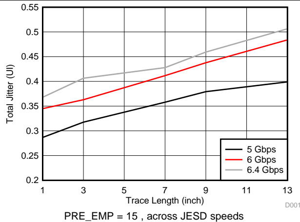
FIG 40. Total Jitter vs Trace Length
