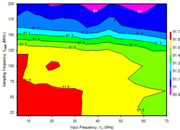
Figure 50. Signal-to-Noise Ratio in 10-Bit, 8-Input Mode
