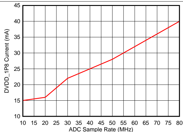
FIG 47. DVDD_1P8 Current vs ADC Sample Rate
