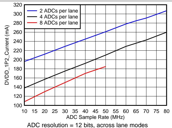
FIG 45. DVDD_1P2 Current vs ADC Sample Rate
