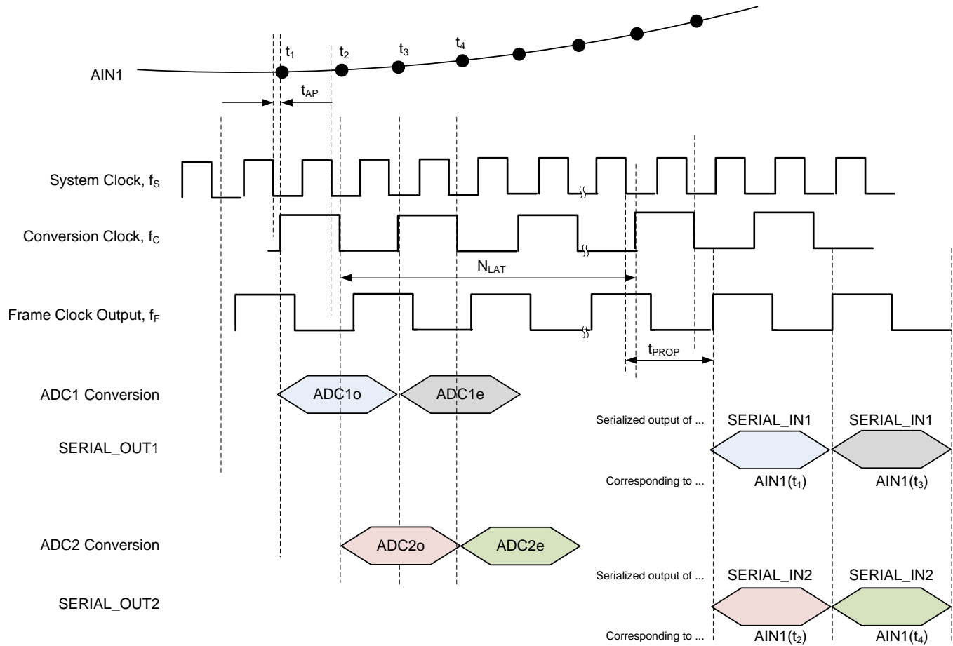
FIG 65. ADC to Output Mapping in 8-Input, 1X Mode in LVDS Interface Mode
