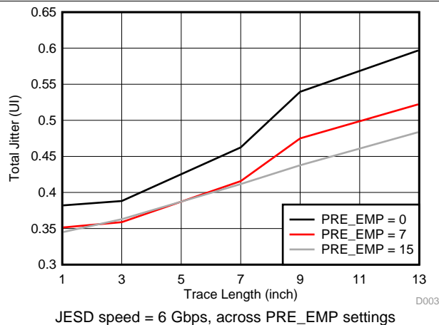
FIG 42. Total Jitter vs Trace Length
