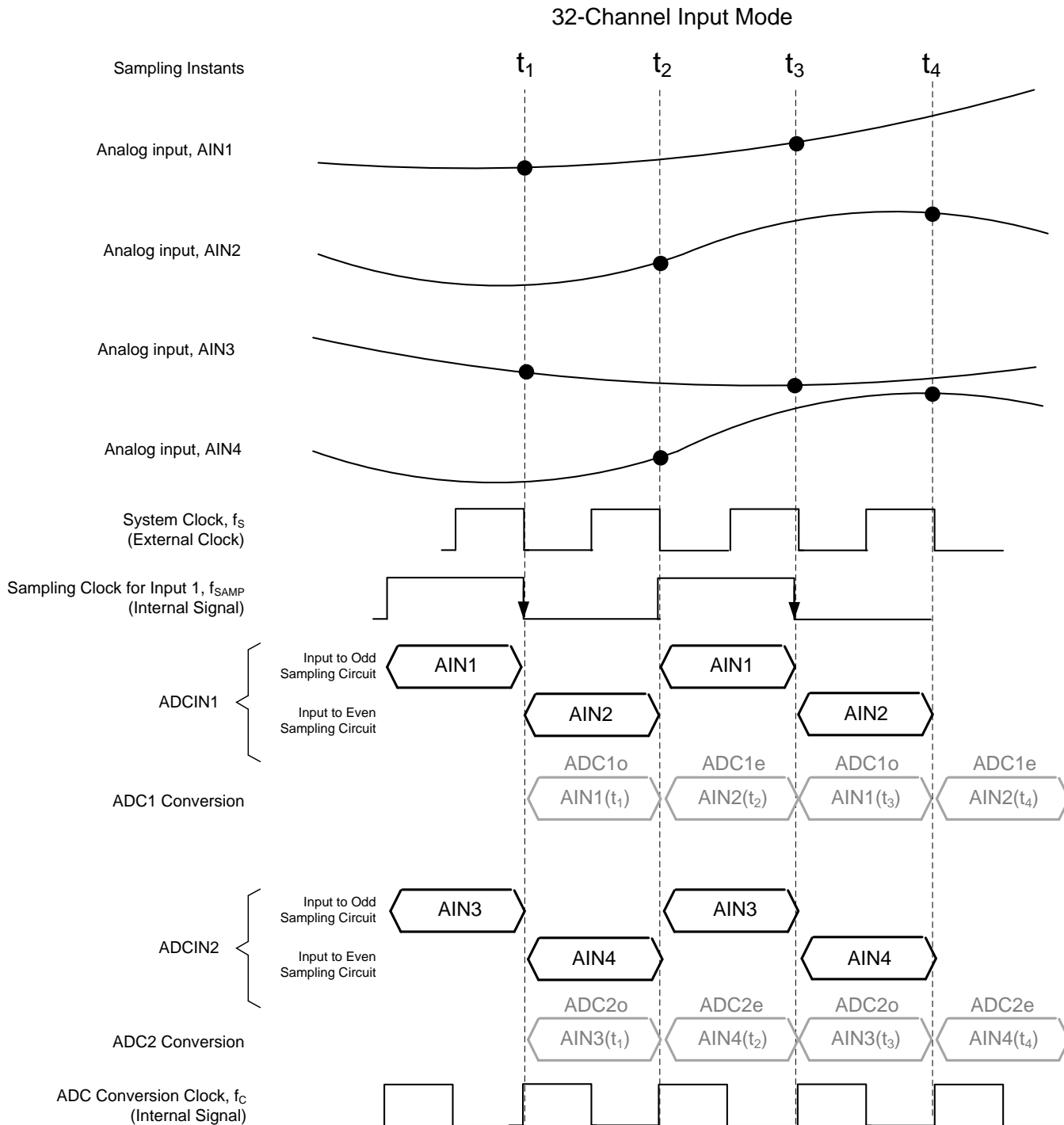
FIG 57. Input Sampling and Conversion Scheme (32-Input Mode)
