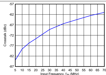
32-input mode, 14-bit resolution, f_{\text{SAMP}} = 32.5 MSPS, –1-dBFS tone applied on one channel and spur on neighboring channel measured as crosstalk
