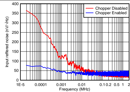
39. Low-Frequency Noise With and Without Chopper Enabled
