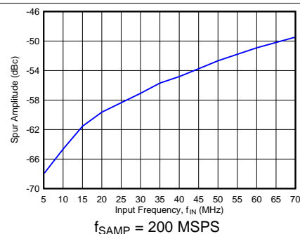
FIG 19. Input-Clock Intermodulation Spur at (f_s / 2 \pm f_{IN}) vs f_{IN} in 8-Input Mode
