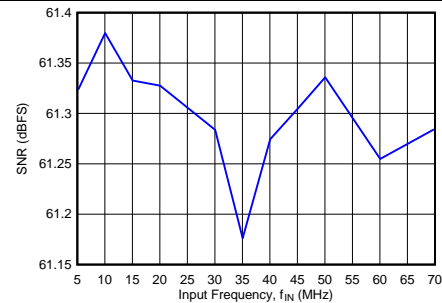
FIG 9. Signal-to-Noise Ratio vs f_{IN} in 10-Bit, 32-Input Mode
