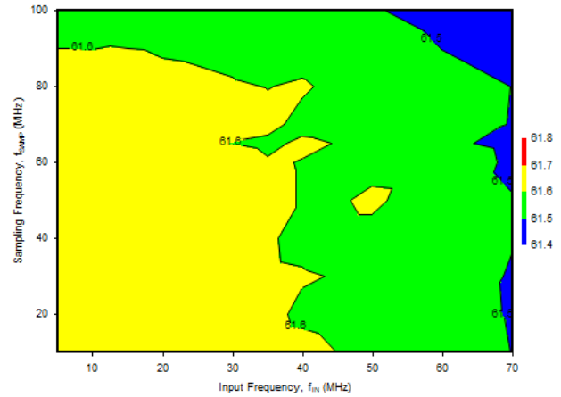
Figure 49. Signal-to-Noise Ratio in 10-Bit, 16-Input Mode
