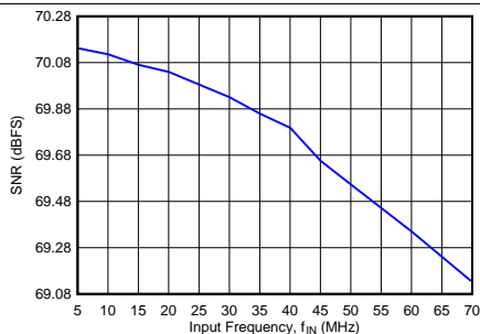
FIG 10. Signal-to-Noise Ratio vs f_{IN} in 10-Bit, 16-Input Mode
