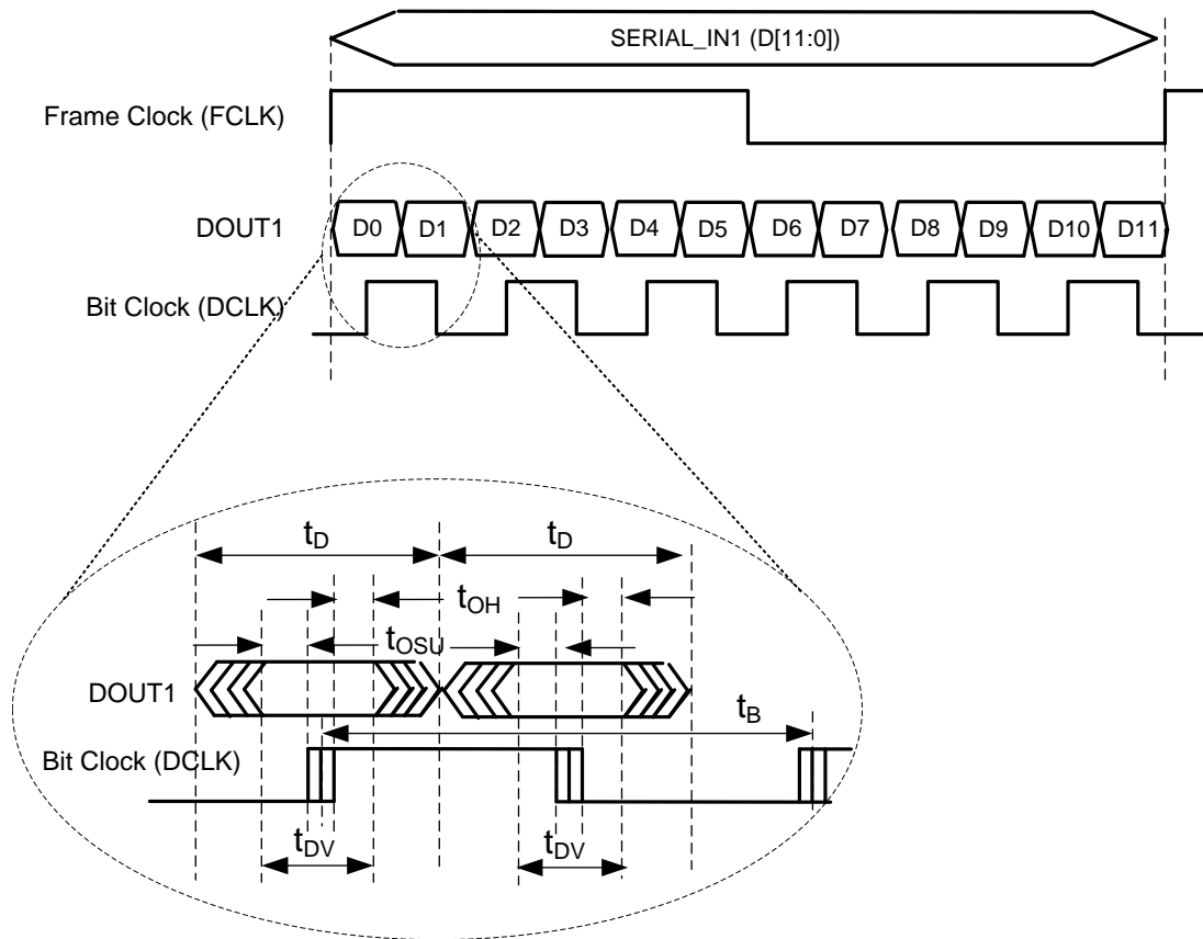
FIG 1. LVDS Output Signals Timing Diagram in 16-Input Mode with 12-Bit Serialization, LSB-First, 1X Data Rate Mode
