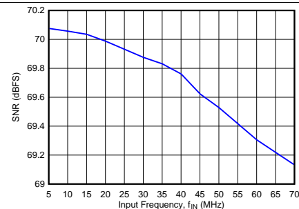
FIG 11. Signal-to-Noise Ratio vs f_{IN} in 10-Bit, 8-Input Mode
