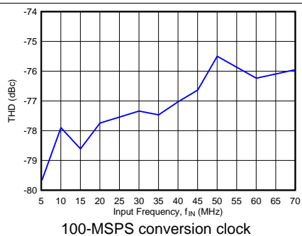
FIG 18. Total Harmonic Distortion vs f_{IN}
