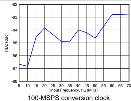
FIG 17. Second-Order Harmonic Distortion vs f_{IN}
