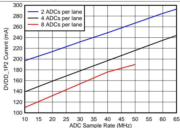
FIG 46. DVDD_1P2 Current vs ADC Sample Rate
