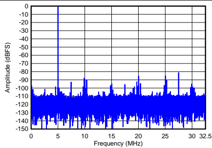
FIG 8. FFT of 14-Bit, 16-Input Mode
