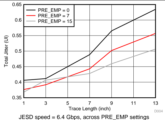
FIG 43. Total Jitter vs Trace Length
