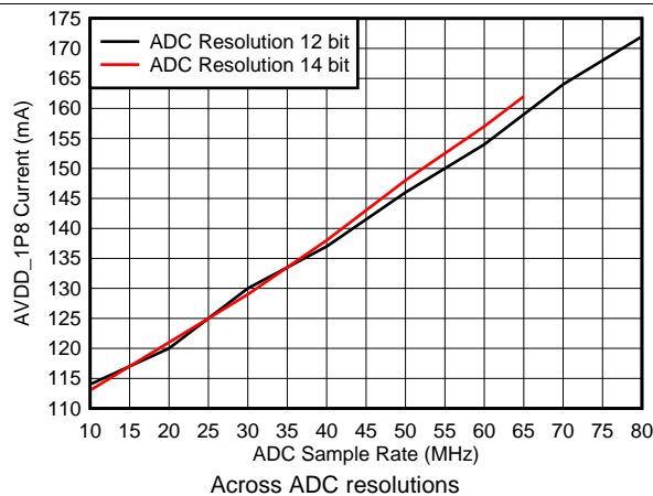
FIG 44. AVDD_1P8 Current vs ADC Sample Rate
