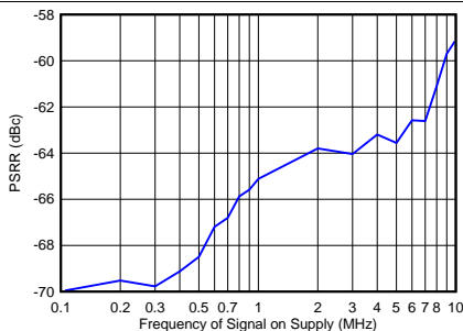
32-input mode, 14-bit resolution, f_{\text{SAMP}} = 32.5 MSPS, 100-mV PP tone on supply
