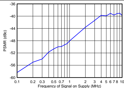
32-input mode; 14-bit resolution; f_{\text{SAMP}} = 32.5 MSPS; 100-mV PP tone on supply; 5-MHz, –1-dBFS tone on input; PSMR is intermodulation tone referred to input tone amplitude
