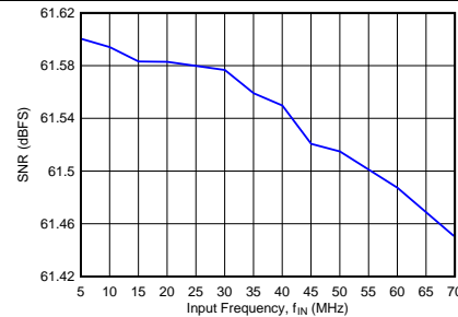
FIG 9. Signal-to-Noise Ratio vs f_{IN} in 10-Bit, 32-Input Mode
