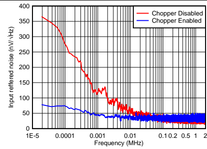
FIG 39. Low-Frequency Noise With and Without Chopper Enabled
