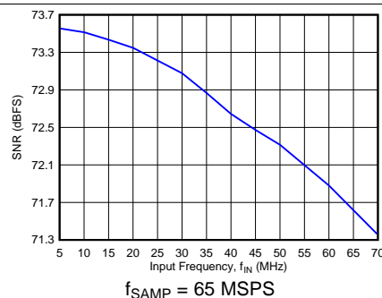
FIG 15. Signal-to-Noise Ratio vs f_{IN} in 14-Bit, 16-Input Mode
