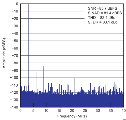
Figure 7. FFT for 3-MHz Input Signal, f_s = 80 MSPS
