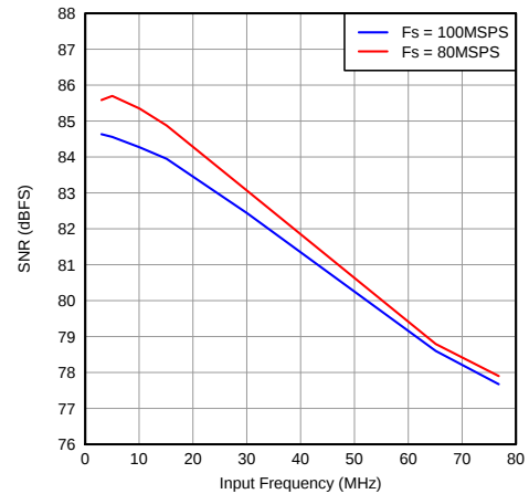
Figure 16. SNR vs Input Frequency
