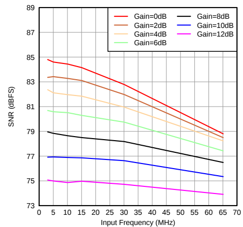
Figure 18. SNR Across Gain
