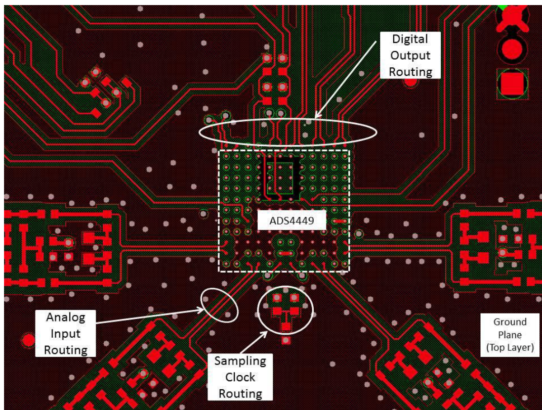
Figure 11-1. ADS4449 Layout
