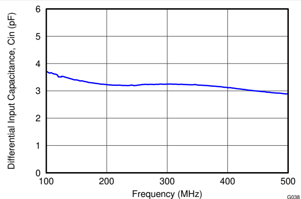
Figure 9-3. ADC Analog Input Capacitance ( C_{IN} ) vs Frequency
