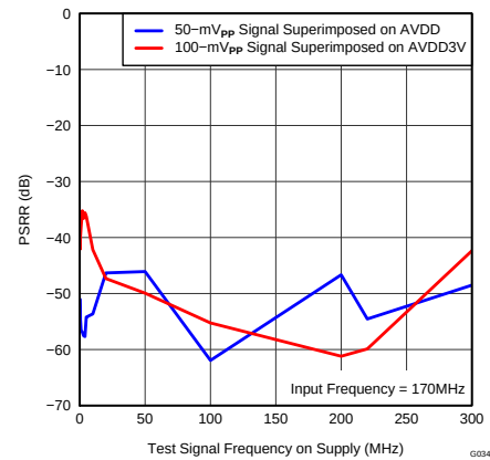
Figure 39. Power-Supply Rejection Ratio vs Test Signal Frequency
