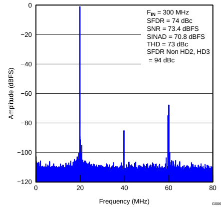
Figure 11. FFT for 300-MHz Input Signal (2.5- V_{PP} Full-Scale)
