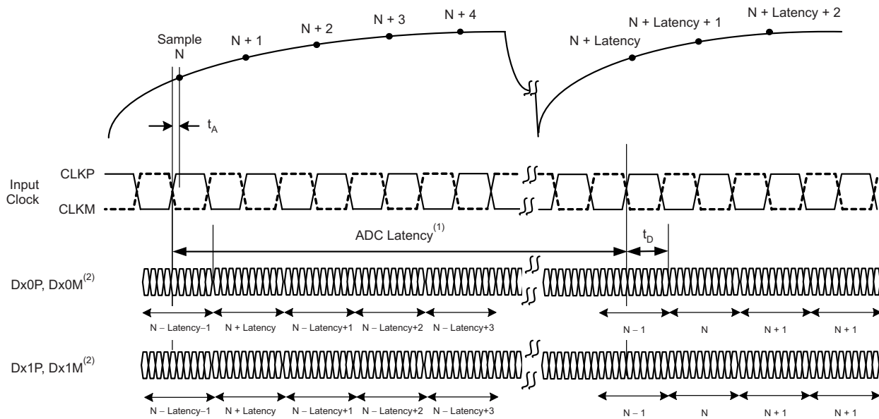
Figure 3. ADC Latency
