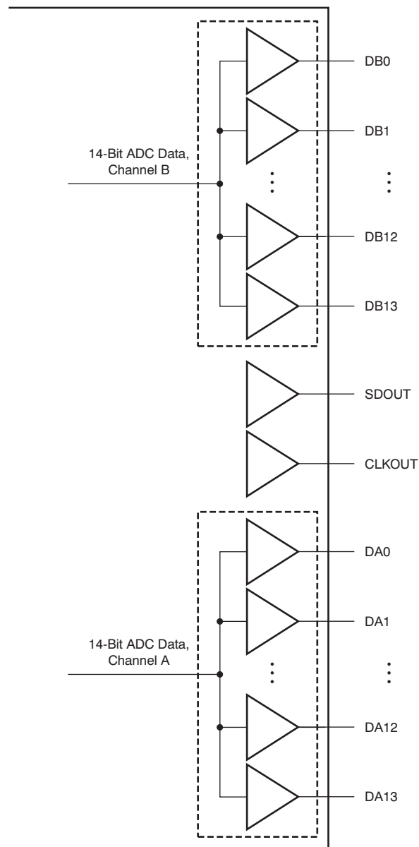
Figure 47. CMOS Outputs
