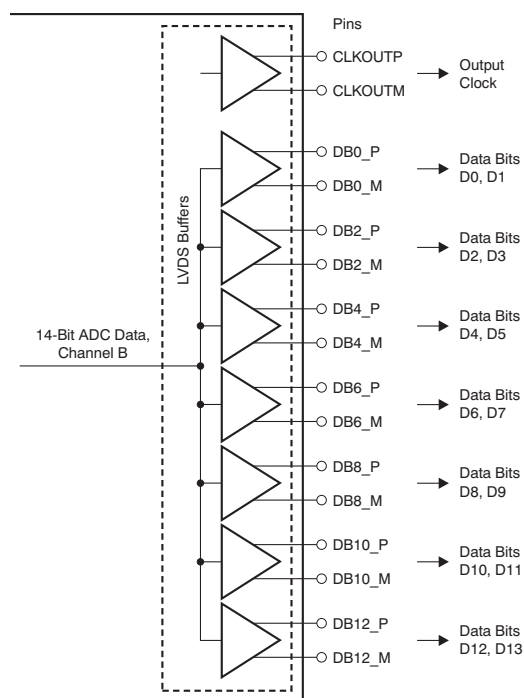
Figure 43. LVDS Interface
