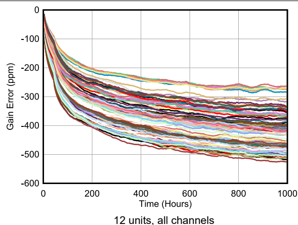
图 6-10. Long-Term Gain Drift
