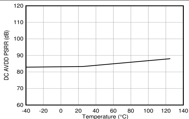
图 6-13. DC AVDD PSRR vs Temperature
