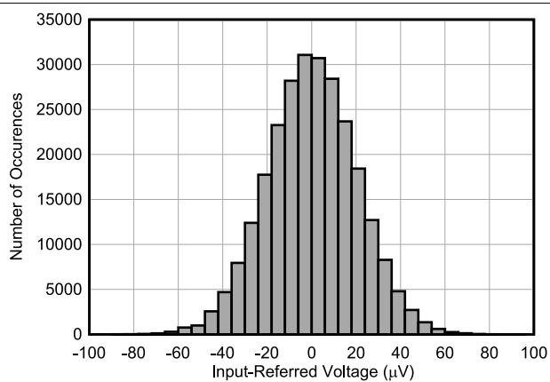
FIG 6-17. Single Device Noise Histogram at 32 kSPS
