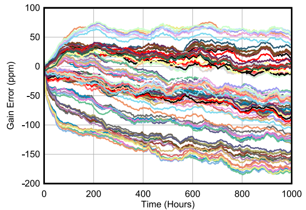
FIG 6-11. Long-Term Gain Drift (WQFN Package)
