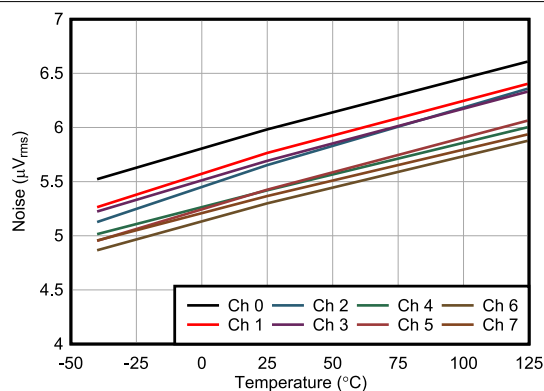
6-17. Noise vs Temperature
