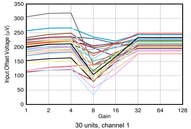
30 units, channel 1 6-7. Input Offset Voltage vs Gain
