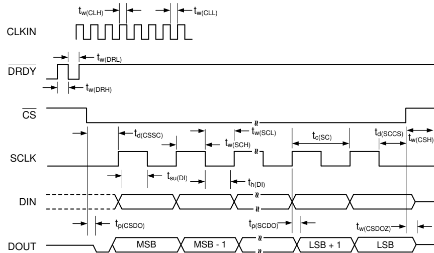
FIG 6-1. SPI Timing Diagram
