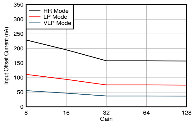
Gains of 8, 16, 32, 64, and 128 only 6-4. Input Offset Current vs Gain
