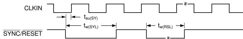
FIG 6-2. SYNC/RESET Timing Requirements
