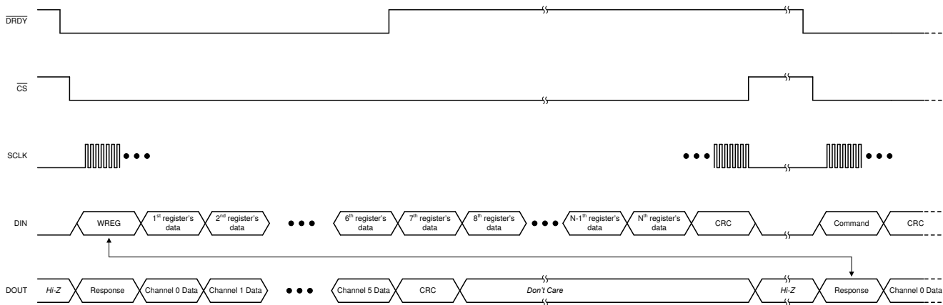
✎ 8-25. Writing Registers
