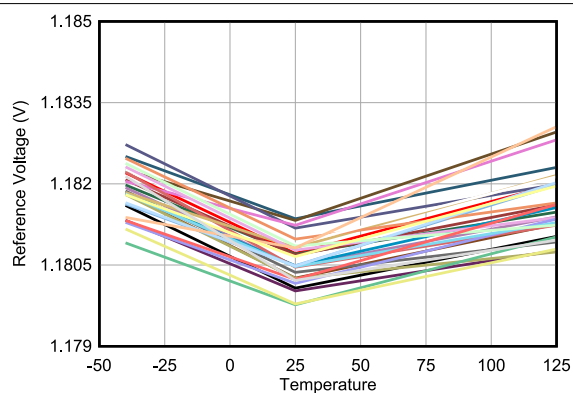
FIG 6-29. Internal Reference Voltage Temperature Drift
