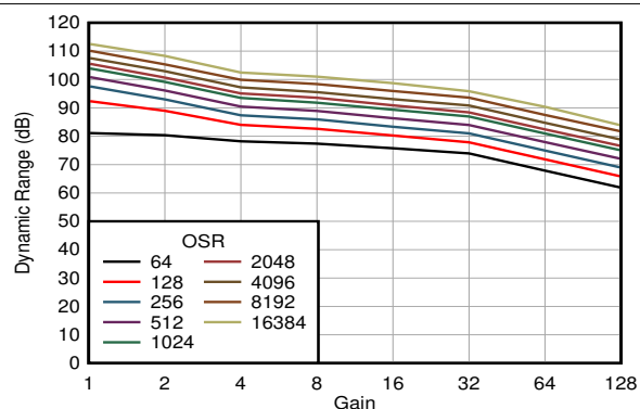
FIG 6-23. Dynamic Range vs Gain
