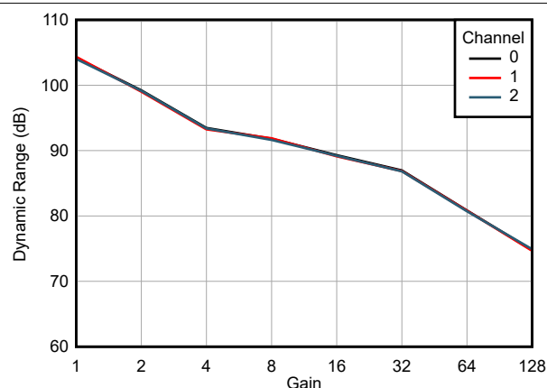
FIG 6-22. Dynamic Range vs Gain
