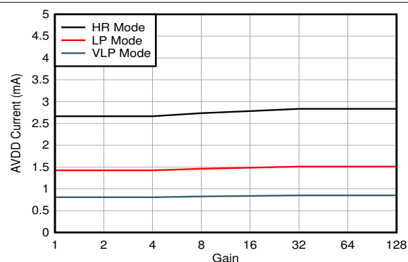
FIG 6-27. AVDD Current vs Gain
