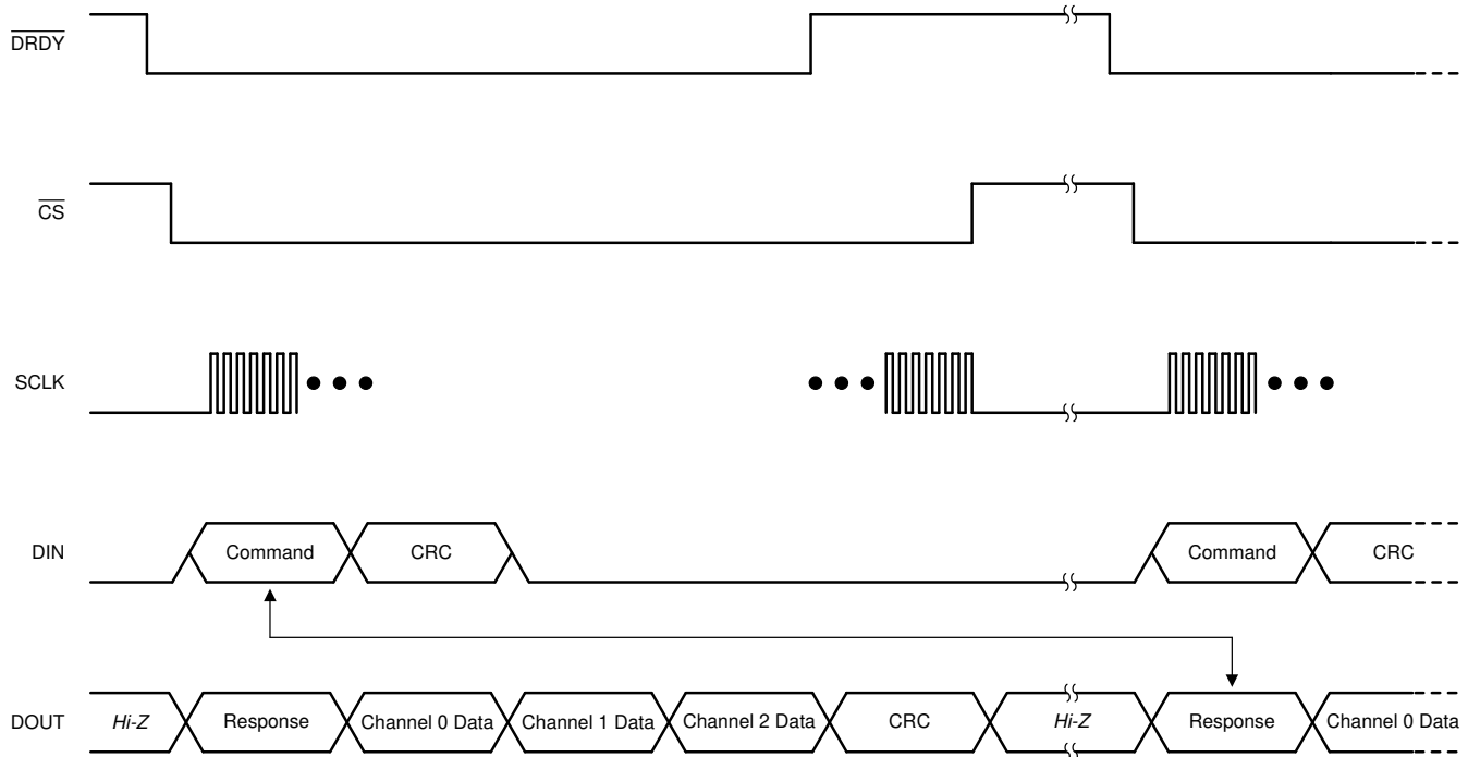
FIG 8-17. Typical Communication Frame
