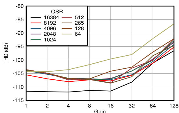
FIG 6-25. THD vs Gain
