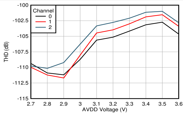
FIG 6-28. THD vs AVDD
