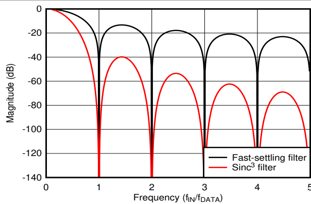
☒ 8-4. Fast-Settling and Sinc 3 Digital Filter Response
