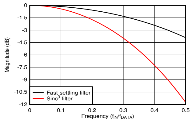
☒ 8-5. Fast-Settling and Sinc 3 Digital Filter Response, Pass-Band Detail
