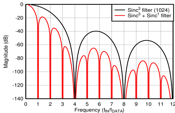
☒ 8-6. Digital Filter Response for OSR = 1024 and OSR = 4096
