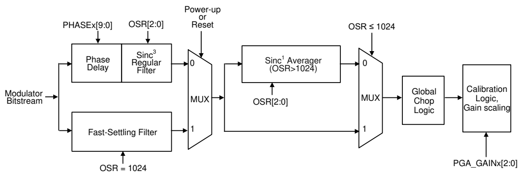
☒ 8-3. Digital Filter Implementation
