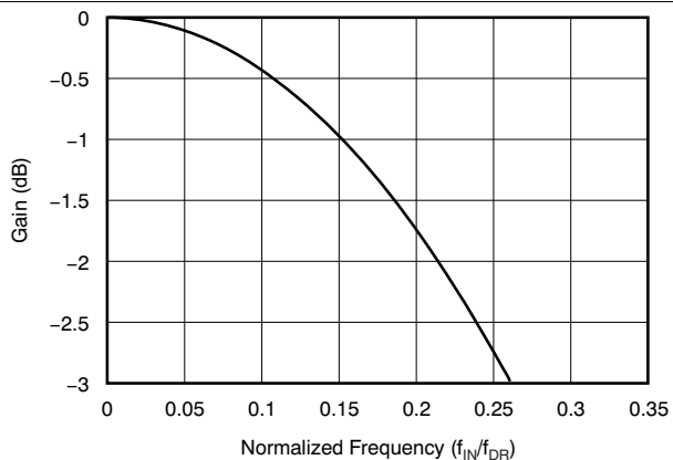
Figure 24. Sinc Filter Roll-Off
