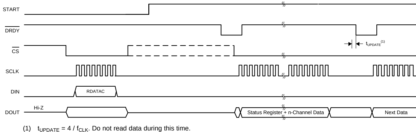
Figure 40. Reading Data in RDATAC Mode
