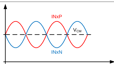
Figure 20. Fully-Differential Input Mode
