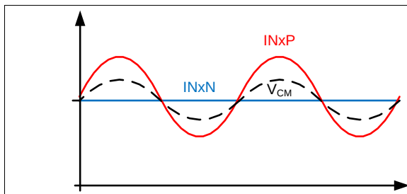
Figure 19. Pseudo-Differential Input Mode
