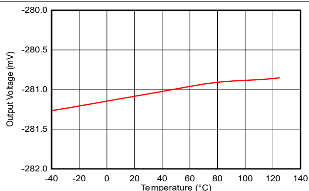
TDACy 出力電圧 = -9 \times V_{\text{REFy}} / 40
