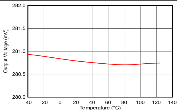
TDACy 出力電圧 = 9 \times V_{\text{REFy}} / 40
