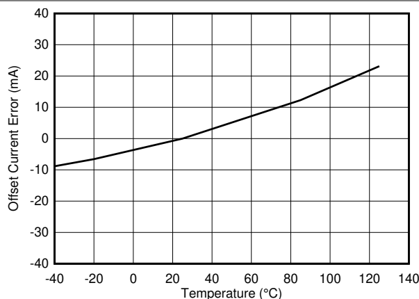
图 9-5. Offset Current Error vs Temperature
