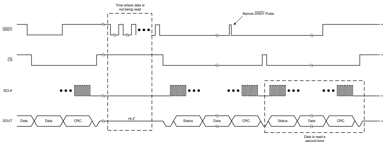
✕ 8-25. Collecting Data After a Pause in Data Collection by Reading Data Twice
