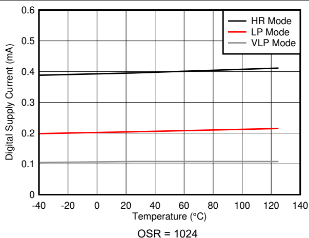
OSR = 1024 6-14. Digital Supply Current vs Temperature
