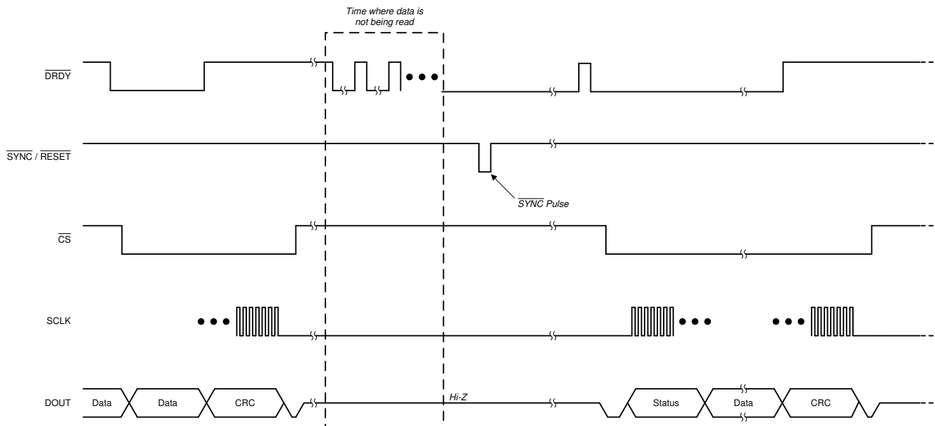
✕ 8-24. Collecting Data After a Pause in Data Collection Using the SYNC/RESET Pin
