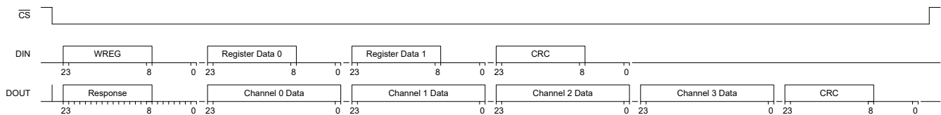
Figure 8-16. SPI Frame using 24-bit Word Size
