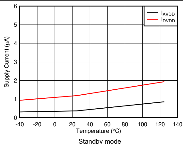
Standby mode 6-15. Supply Current vs Temperature
