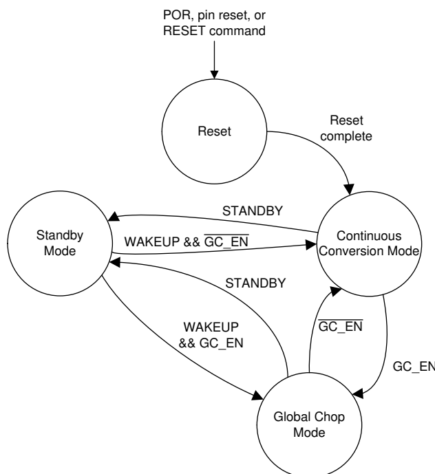
8-10. State Diagram Depicting Device Functional Modes
