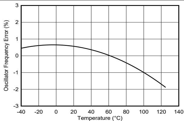
6-11. Oscillator Frequency Error vs Temperature
