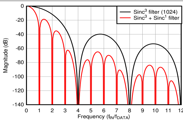
Figure 8-7. Digital Filter Response for OSR = 1024 and OSR = 4096
