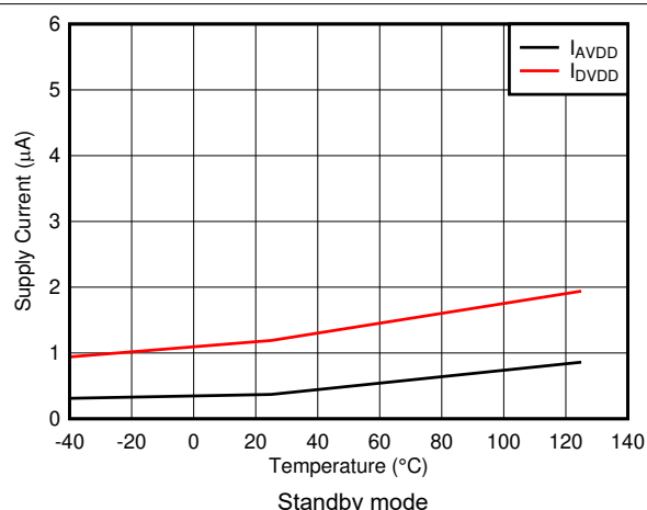
6-15. Supply Current vs Temperature
