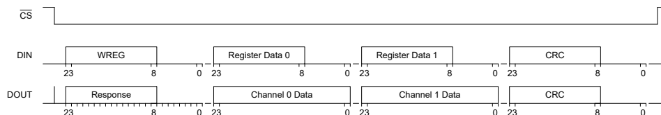
Figure 8-16. SPI Frame using 24-bit Word Size
