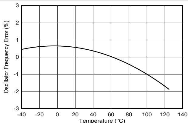
6-11. Oscillator Frequency Error vs Temperature
