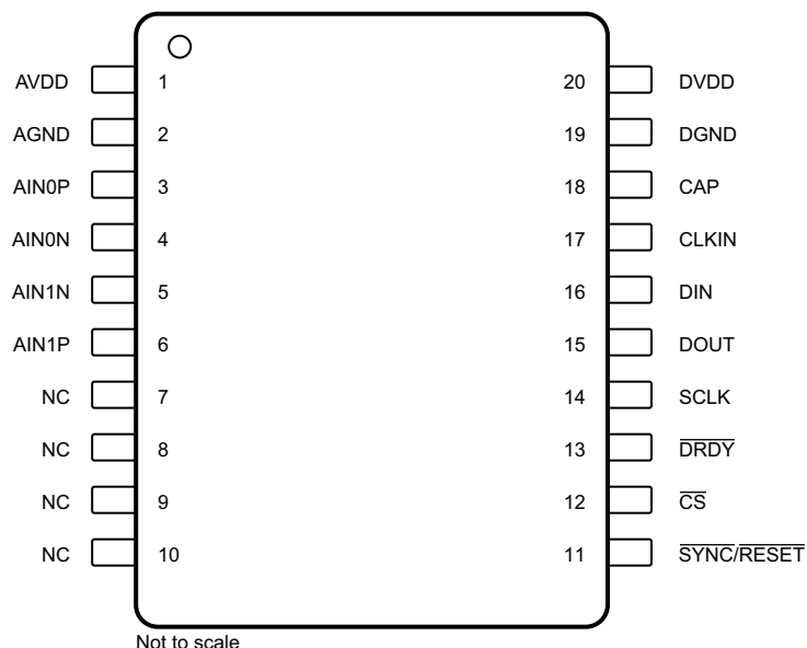
图 5-1. PW Package, 20-Pin TSSOP, Top View
