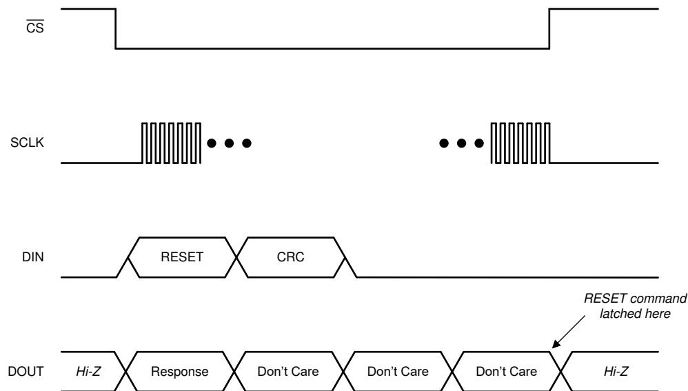
FIG 8-20. RESET Command Frame
