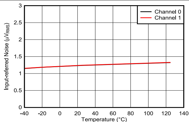
6-10. Input-referred Noise vs Temperature
