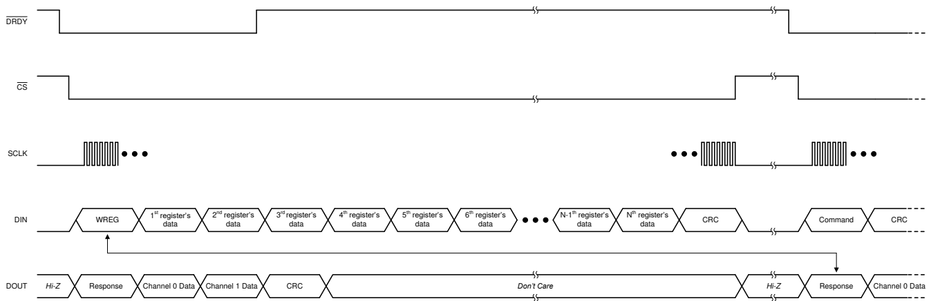
✎ 8-23. Writing Registers
