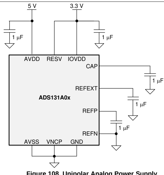
Figure 108. Unipolar Analog Power Supply
