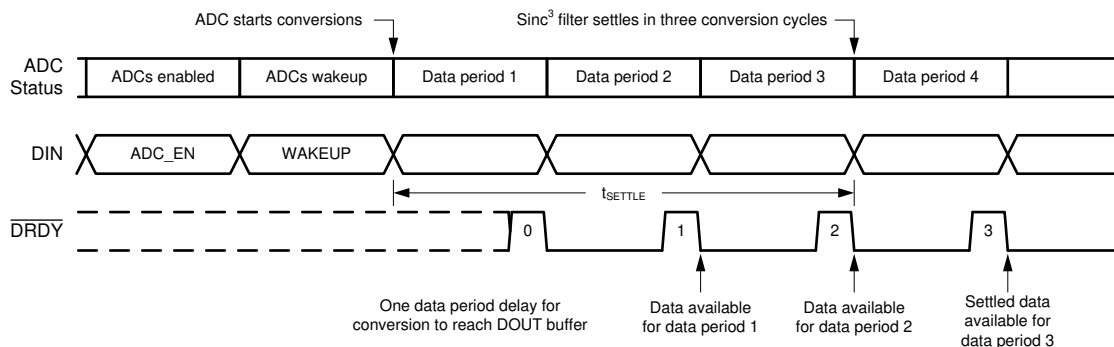
Figure 51. \text{Sinc}^3 Filter Settling
