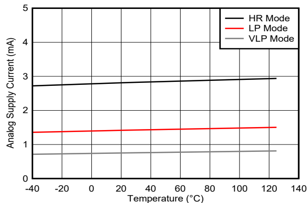
图 6-11. Analog Supply Current vs Temperature
