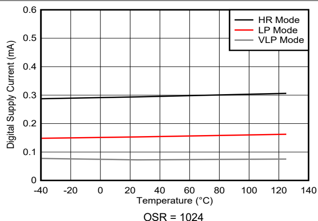
图 6-13. Digital Supply Current vs Temperature
