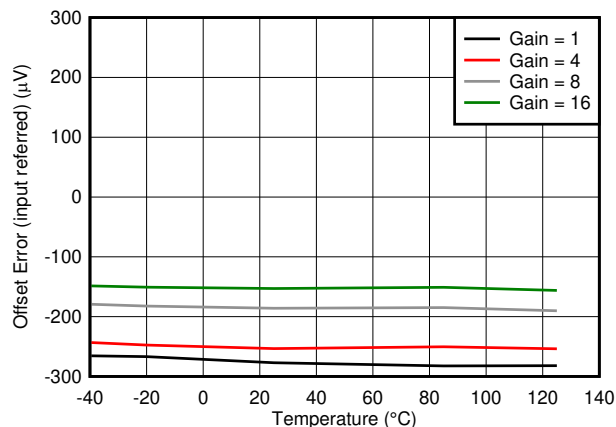
FIG 6-6. Offset Error vs Temperature
