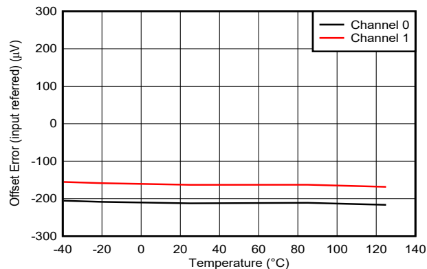
FIG 6-4. Offset Error vs Temperature
