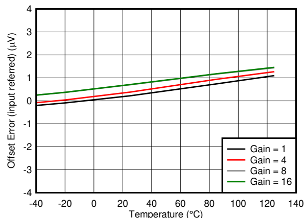
FIG 6-5. Offset Error vs Temperature
