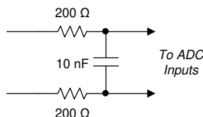
図 9-1. Antialias Filter Example
