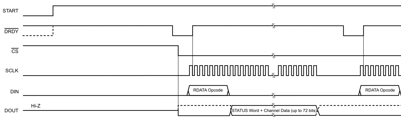
Figure 53. RDATA Usage
