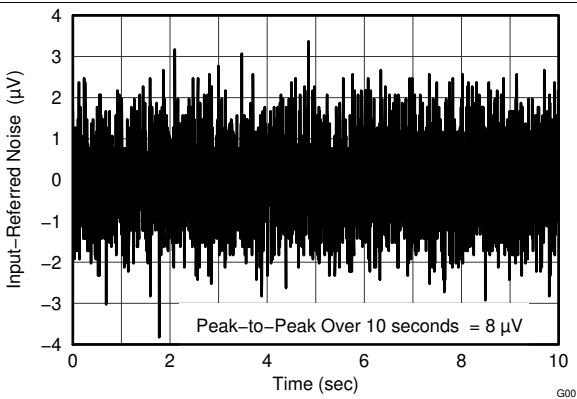
Figure 2. Input-Referred Noise
