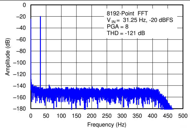
Figure 15. Output Spectrum
