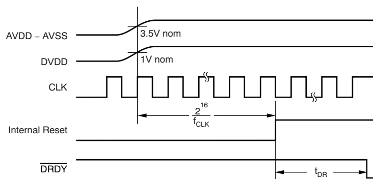
Figure 57. Power-On Sequence
