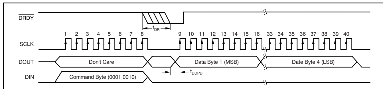
Figure 57. Read Data by Command, RDATA ( t_{\text{DR}} Timing is Given in Table 14)
