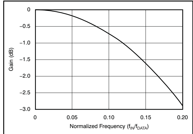
Figure 39. Sinc Filter Roll-Off
