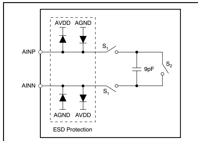
Figure 64. Equivalent Analog Input Circuitry
