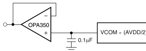
Figure 84. VCOM Output
