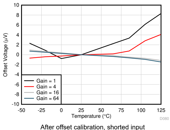
7-50. ADC2 Offset Voltage vs Temperature
