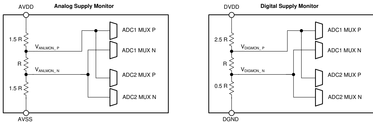
Figure 9-5. Power-Supply Monitors
