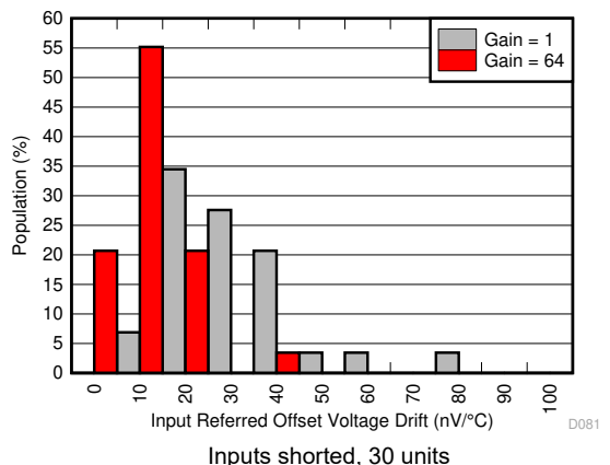
7-51. ADC2 Offset Voltage vs Temperature Distribution
