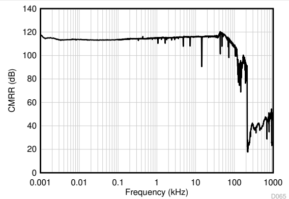
FIG 7-35. ADC1 CMRR vs Frequency
