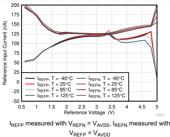
FIG 7-34. ADC1 Reference Input Current
