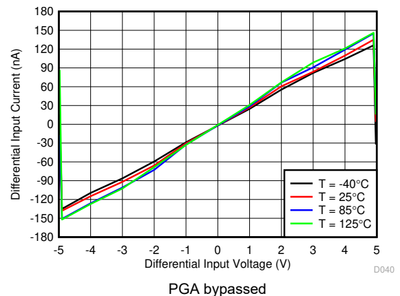
7-25. ADC1 Differential Input Current
