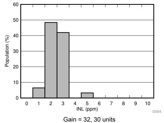
7-23. ADC1 INL Distribution
