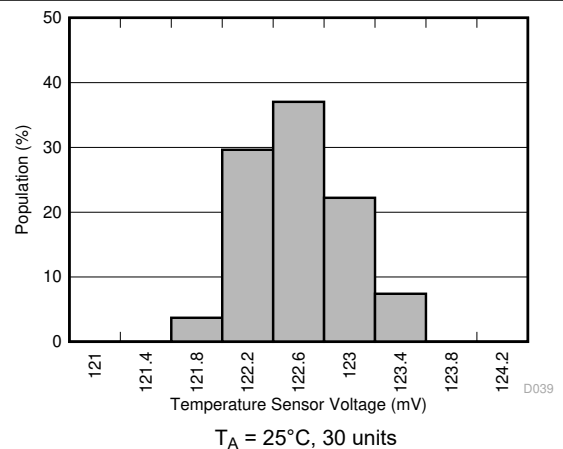
7-43. Temperature Sensor Voltage Distribution
