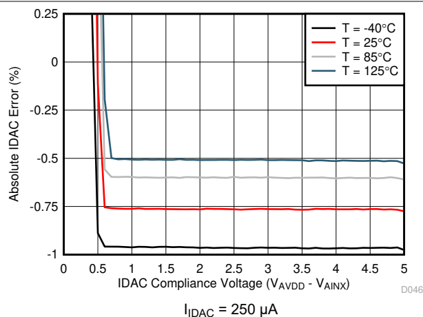
FIG 7-38. IDAC Error vs Compliance Voltage
