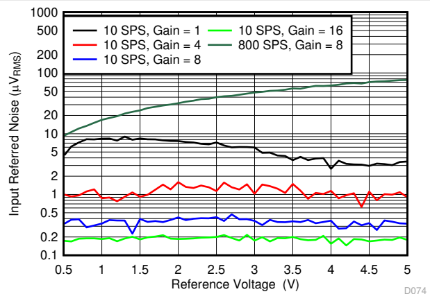
7-59. ADC2 Noise vs Reference Voltage
