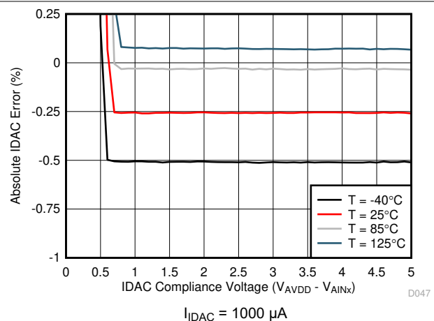
FIG 7-39. IDAC Error vs Compliance Voltage
