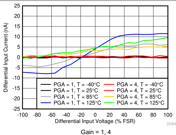
7-62. ADC2 Differential Input Current
