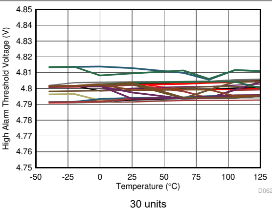
7-48. ADC1 Absolute High Alarm Threshold vs Temperature
