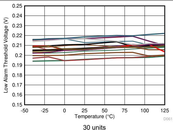
7-47. ADC1 Absolute Low Alarm Threshold vs Temperature
