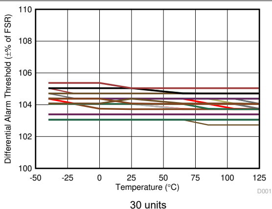
7-46. ADC1 Differential Over-range Alarm Threshold vs Temperature
