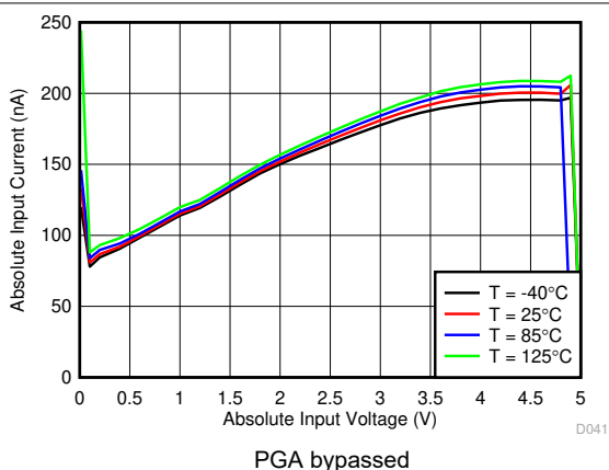
7-26. ADC1 Absolute Input Current
