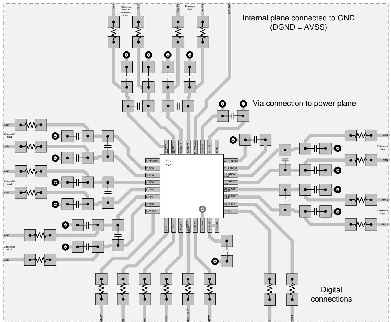
121. ADS124S0x Layout Example
