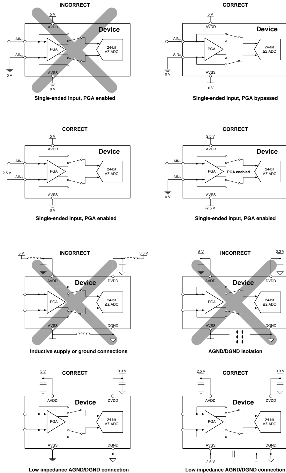
☒ 117. Do's and Don'ts Circuit Connections
