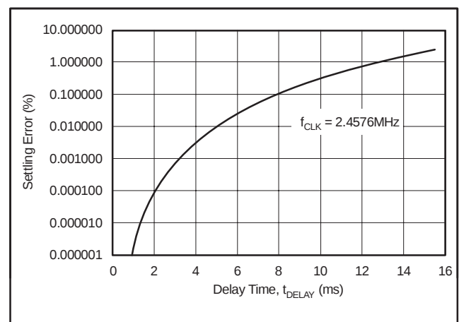
Figure 21. Settling Error vs Delay Time
