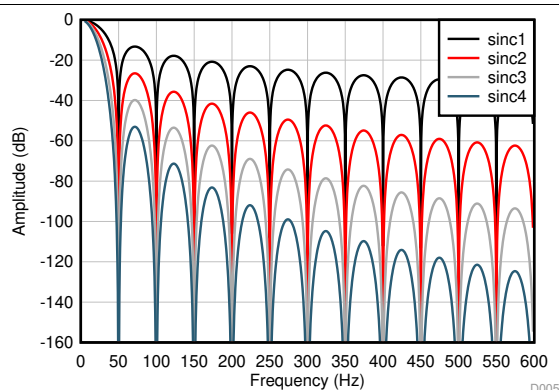
Figure 51. Sinc Frequency Response (50 SPS)
