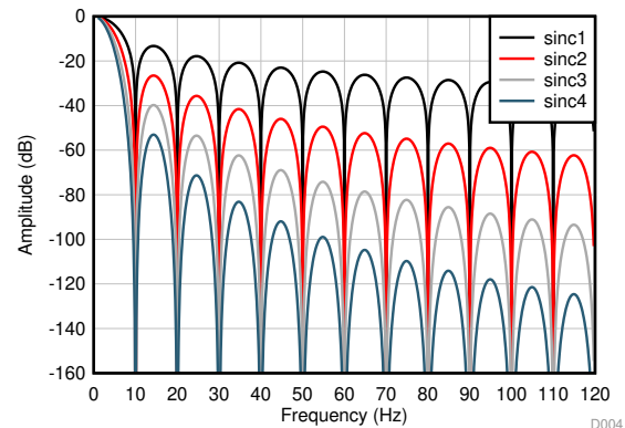
Figure 50. Sinc Frequency Response (10 SPS)
