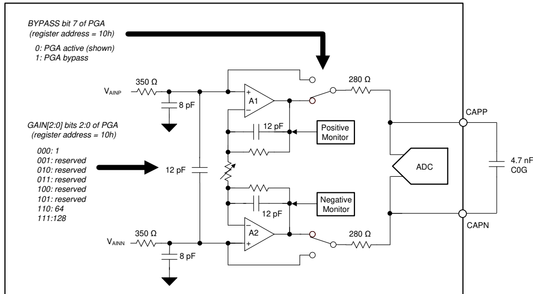
40. PGA Block Diagram
