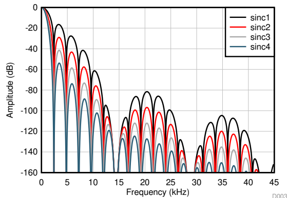
Figure 49. Sinc Frequency Response (2400 SPS)
