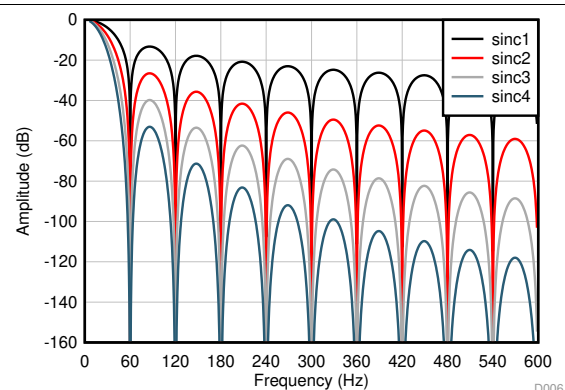
Figure 52. Sinc Frequency Response (60 SPS)
